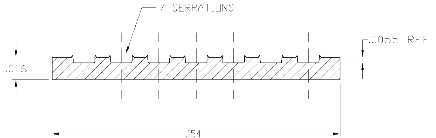
TYP. CROSS SECTION
