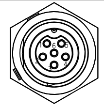
6 Pin
