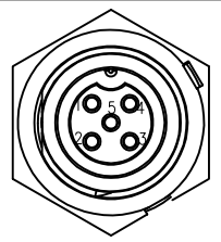
5 Pin
