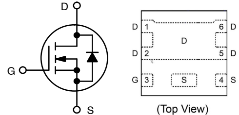
N-CHANNEL MOSFET
