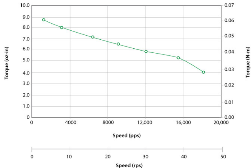
211-18-02 24VDC, 1.3 Amps/Phase, Bipolar, 1/2 Stepping
