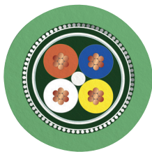
PROFINET stranded CAT5 [93M]
