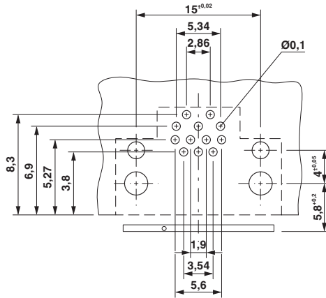
Drilling diagram
