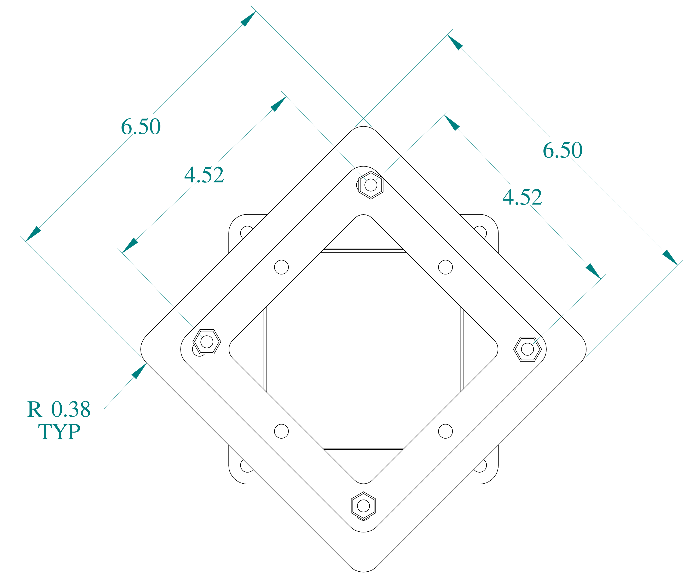
BACK VIEW
