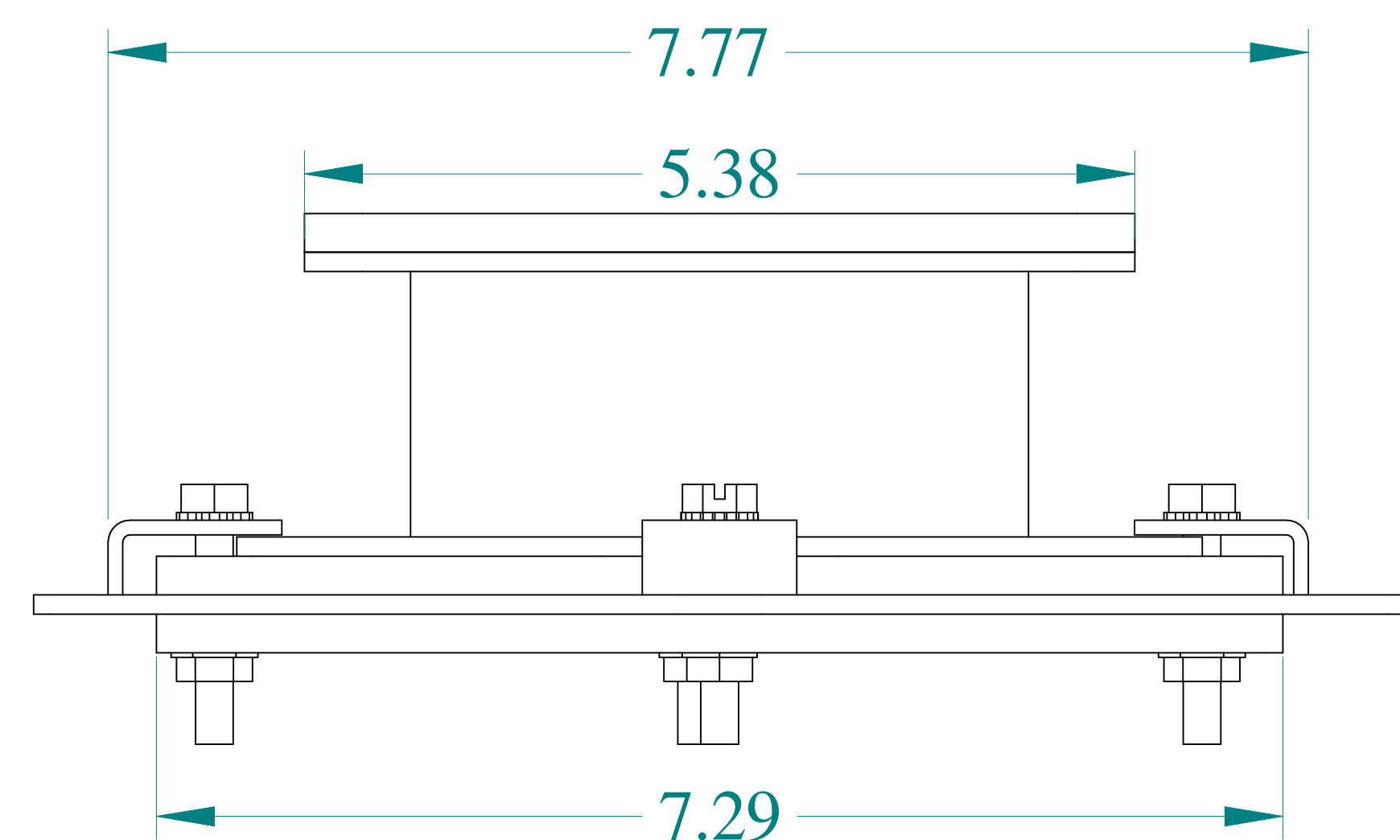
BOTTOM VIEW
