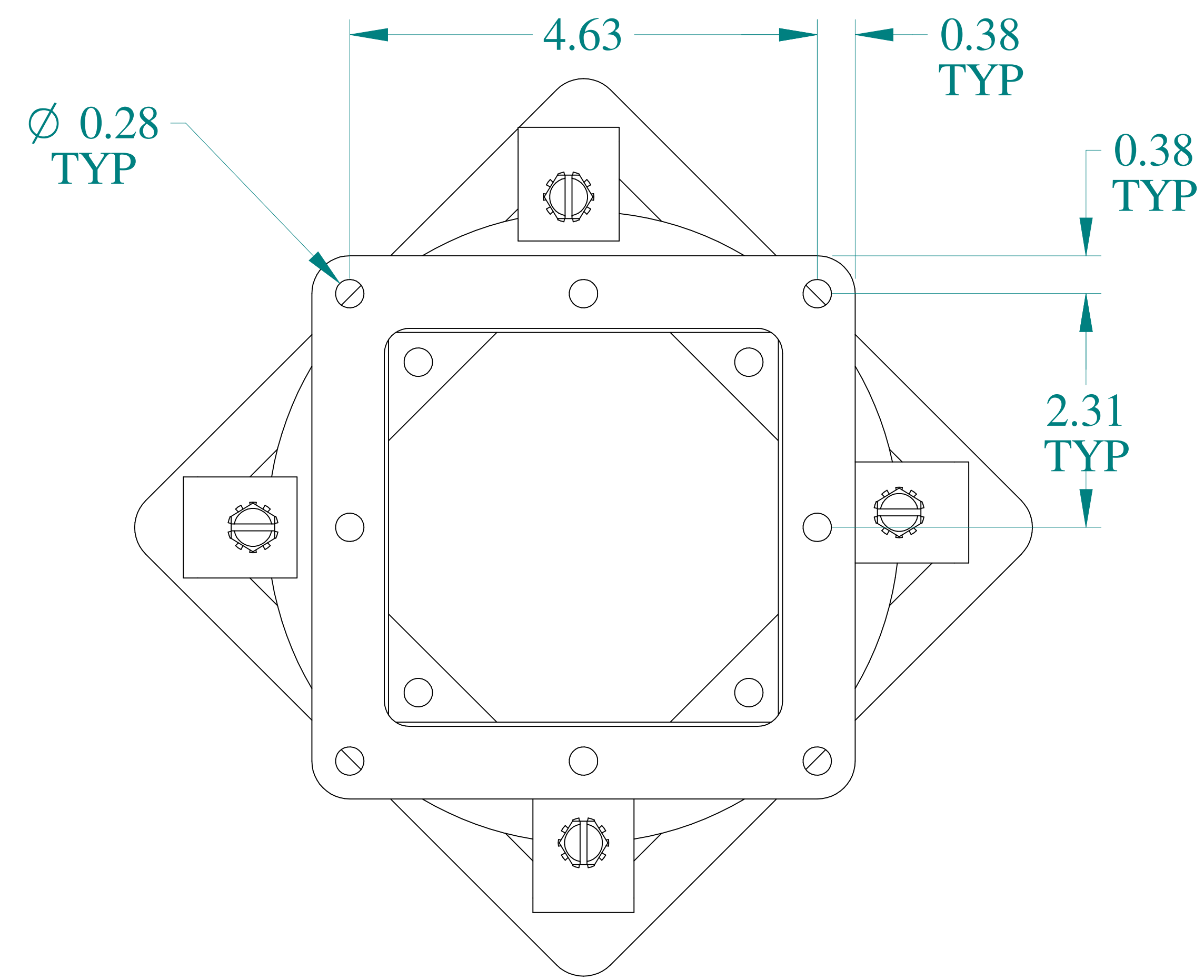
FRONT VIEW
