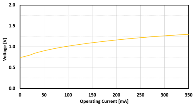
FIG. 13: SLED 2 FORWARD VOLTAGE VS CURRENT
