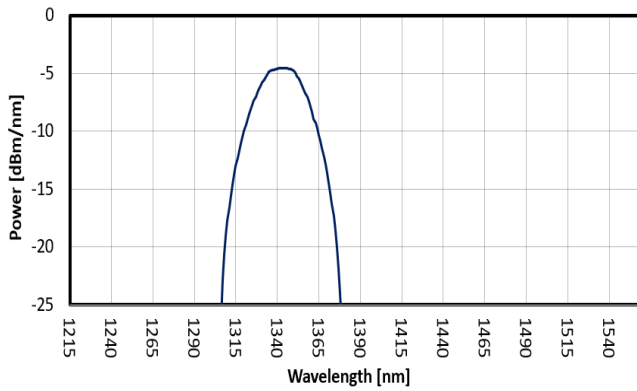
FIG. 5: SLED 4 SPECTRUM
