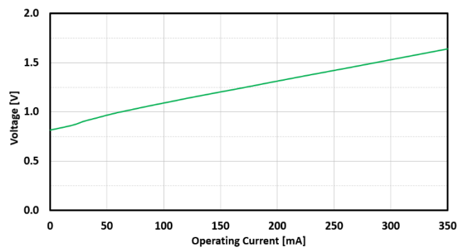
FIG. 12: SLED 1 FORWARD VOLTAGE VS CURRENT
