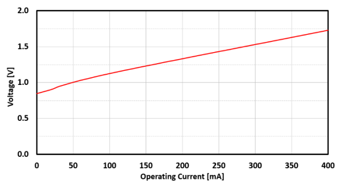
FIG. 14: SLED 3 FORWARD VOLTAGE VS CURRENT
