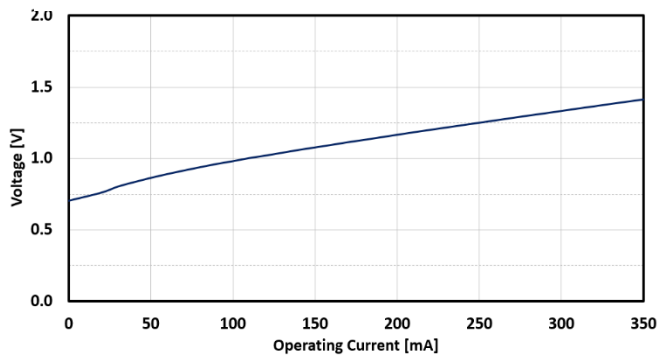
FIG. 15: SLED 4 FORWARD VOLTAGE VS CURRENT
