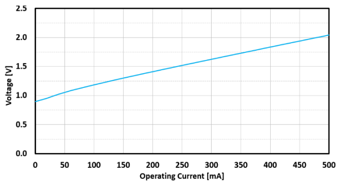
FIG. 16: SLED 5 FORWARD VOLTAGE VS CURRENT
