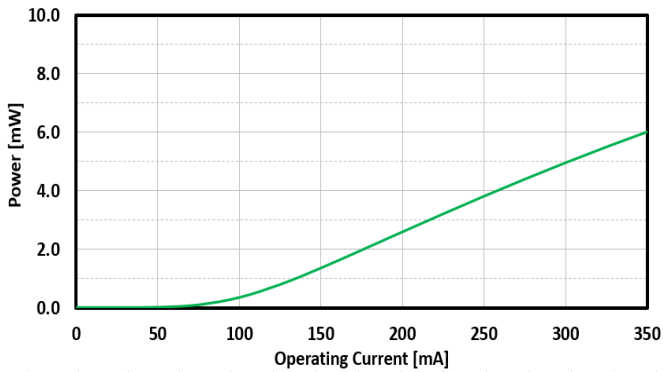
FIG. 7: SLED 1 OUTPUT POWER VS CURRENT
