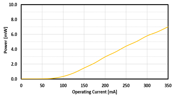
FIG. 8: SLED 2 OUTPUT POWER VS CURRENT
