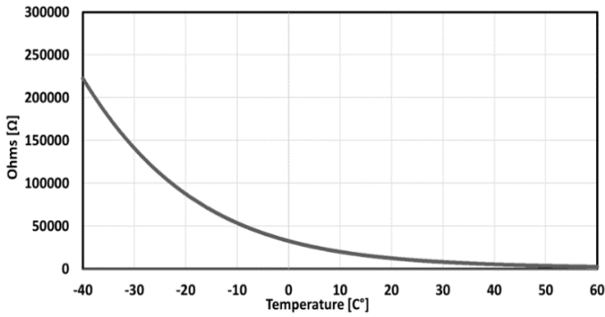
FIG. 17: THERMISTOR R_{THTEC} RESISTANCE VS TEMPERATURE
