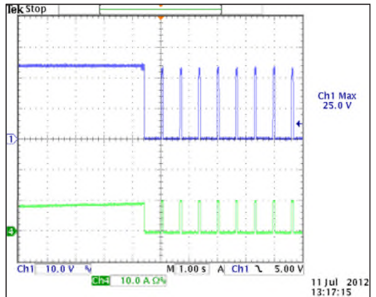
24V OUT, 264VAC
