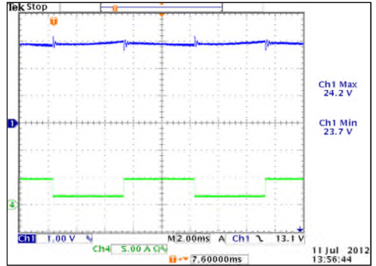
24V OUT, 240VAC, 25% TO 75% LOAD STEP
