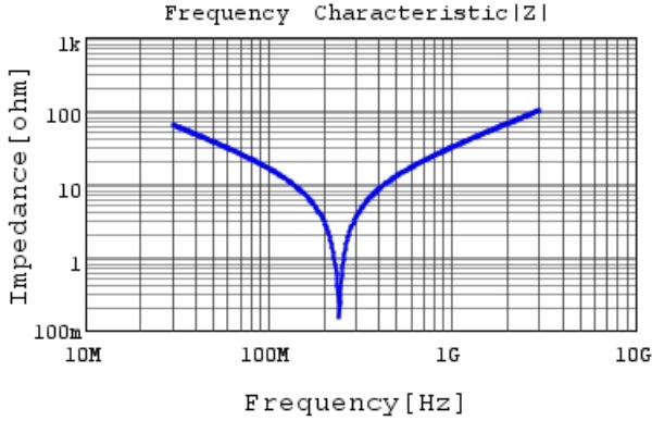
RCE5C2E820J1K1H03B |Z| DC0V, 25degC
