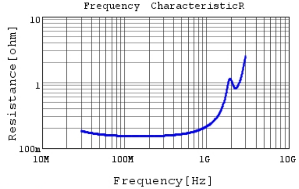
RCE5C2E820J1K1H03B R DC0V, 25degC
