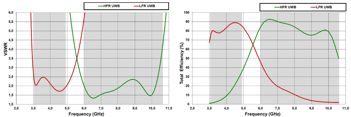
Figure 14 – VSWR and total efficiency for the UWB LFR (3.1GHz – 4.8GHz) and for the UWB HFR (6.0GHz – 10.6GHz) from the Evaluation Board (
