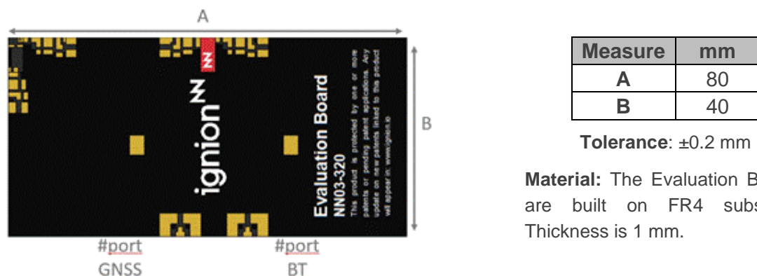
Figure 1 – EB_NN03-320-m-GNSS-BT Evaluation Board providing operation at BeiDou E1 band (1561 MHz), GPS L1 band and GALILEO E1 band (1575 MHz), GLONASS L1 band (from 1598 MHz to 1606 MHz) and Bluetooth (from 2400MHz to 2480MHz). Notice that the clearance area is equal to the DUO mXTEND ™ footprint.
