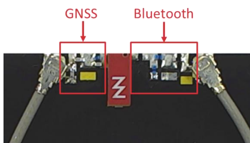
Figure 2 – Matching network distribution in the Evaluation Board ( Error! Reference source not found. ).
