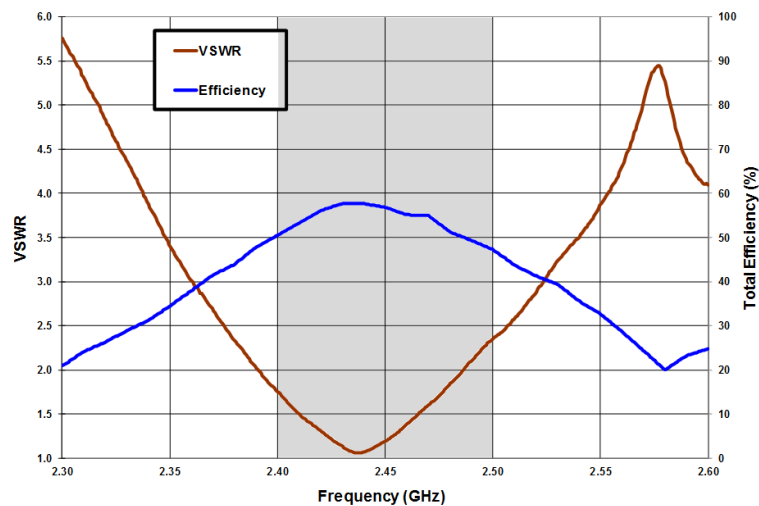
Figure 5 – VSWR and Total Efficiency for the 2400 – 2500 MHz (from the Evaluation Board) ( Error! Reference source not found. ).
