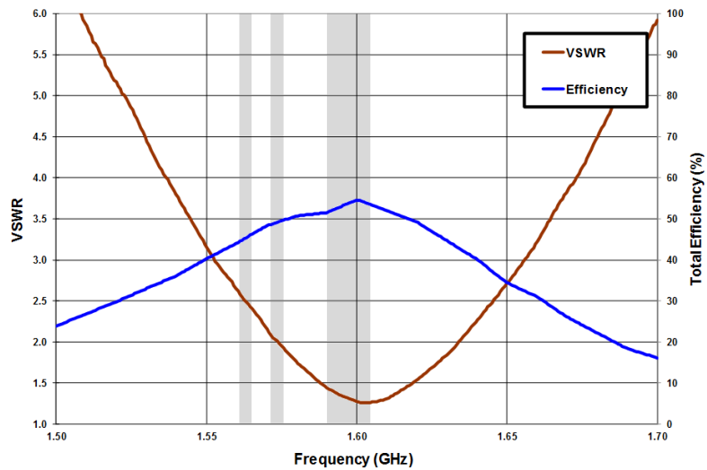
Figure 4 – VSWR and Total Efficiency at BeiDou E1 band (1561 MHz), GPS L1 band and GALILEO E1 band (1575 MHz), GLONASS L1 band (from 1598 to 1606 MHz) (from the Evaluation Board) ( Error! Reference source not found. ).
