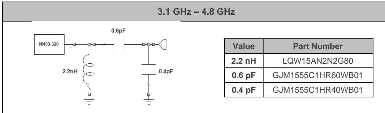
Figure 12 – Matching network implemented in the Evaluation Board (
