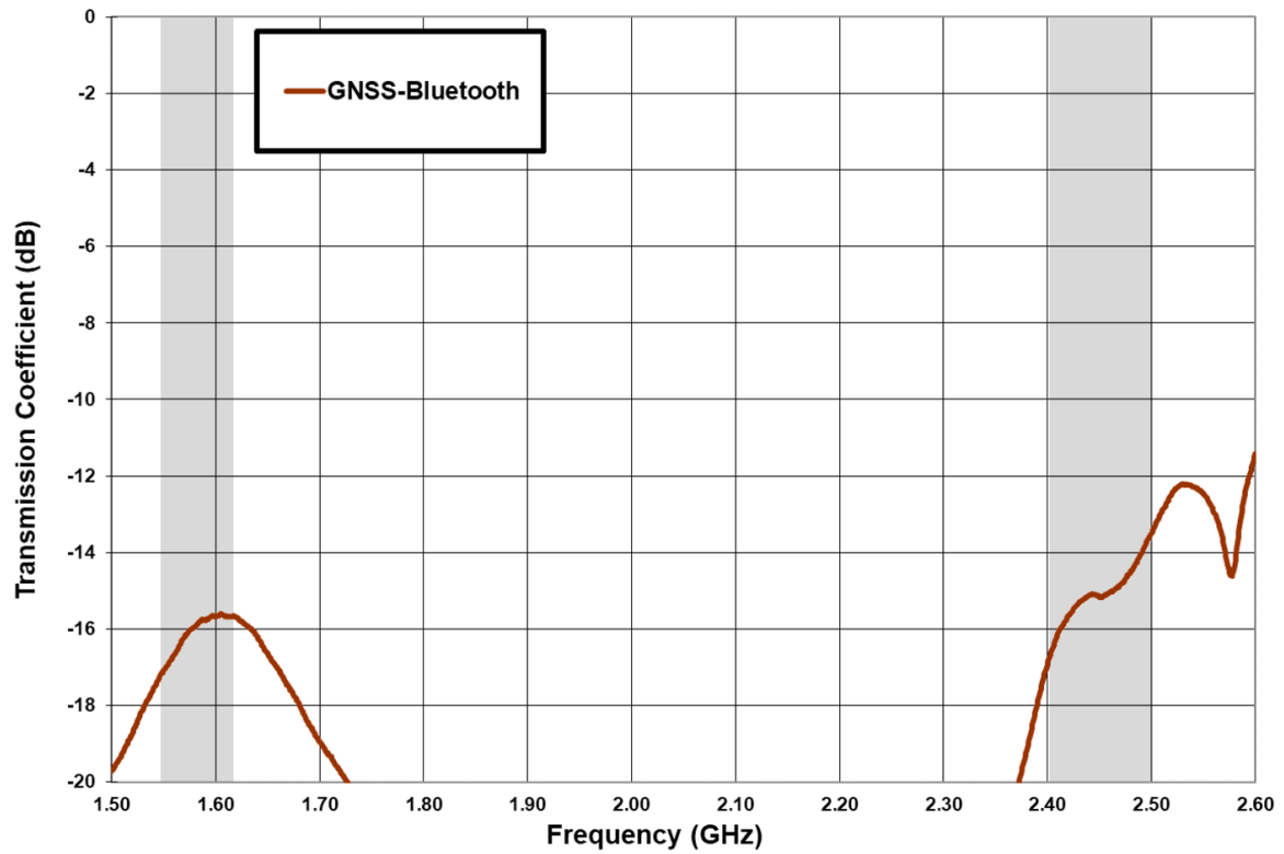
Figure 6 – Transmission coefficient between GNSS (1561 – 1606 MHz) and Bluetooth (2400 – 2500 MHz) from the Evaluation Board ( Error! Reference source not found. ).
