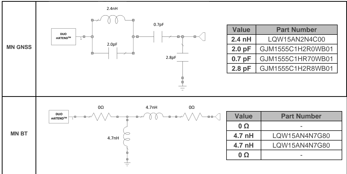
Figure 3 – Matching network implemented in the Evaluation Board 1 port ( Error! Reference source not found. ).
