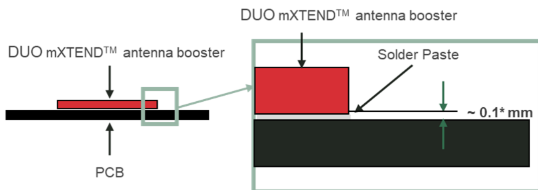
Figure 19 – Soldering Details.
