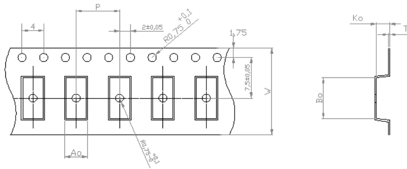
Figure 21 – Tape dimensions and tolerances.
