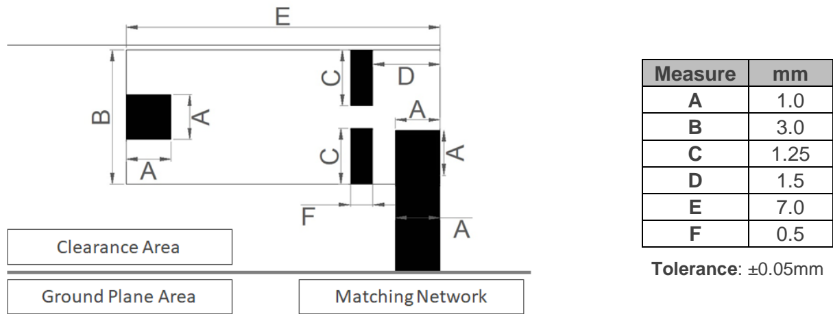
Figure 15 – Footprint dimensions for the NN03-320 in the corner for UWB.
