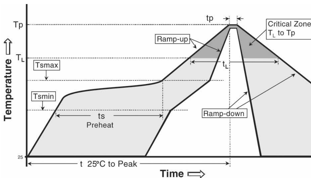
Figure 20 – Temperature profile.
