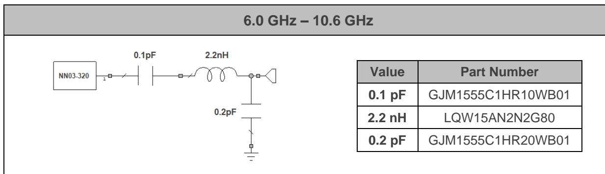
Figure 13 – Matching network implemented in the Evaluation Board (
