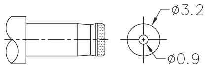
MATING PLUG Jack Insertion Depth: 7.0 mm
