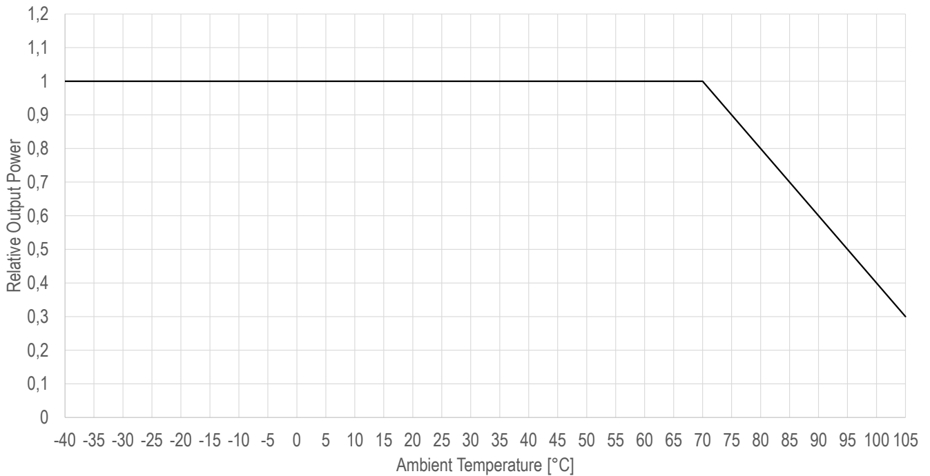
1769405241, 1769405341 Output Power Thermal Derating Nominal V_{IN} , I_{OUT} = 0.4A
