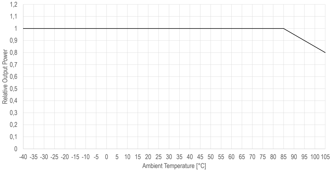
1769405141 Output Power Thermal Derating Nominal V_{IN} , I_{OUT} = 0.4A
