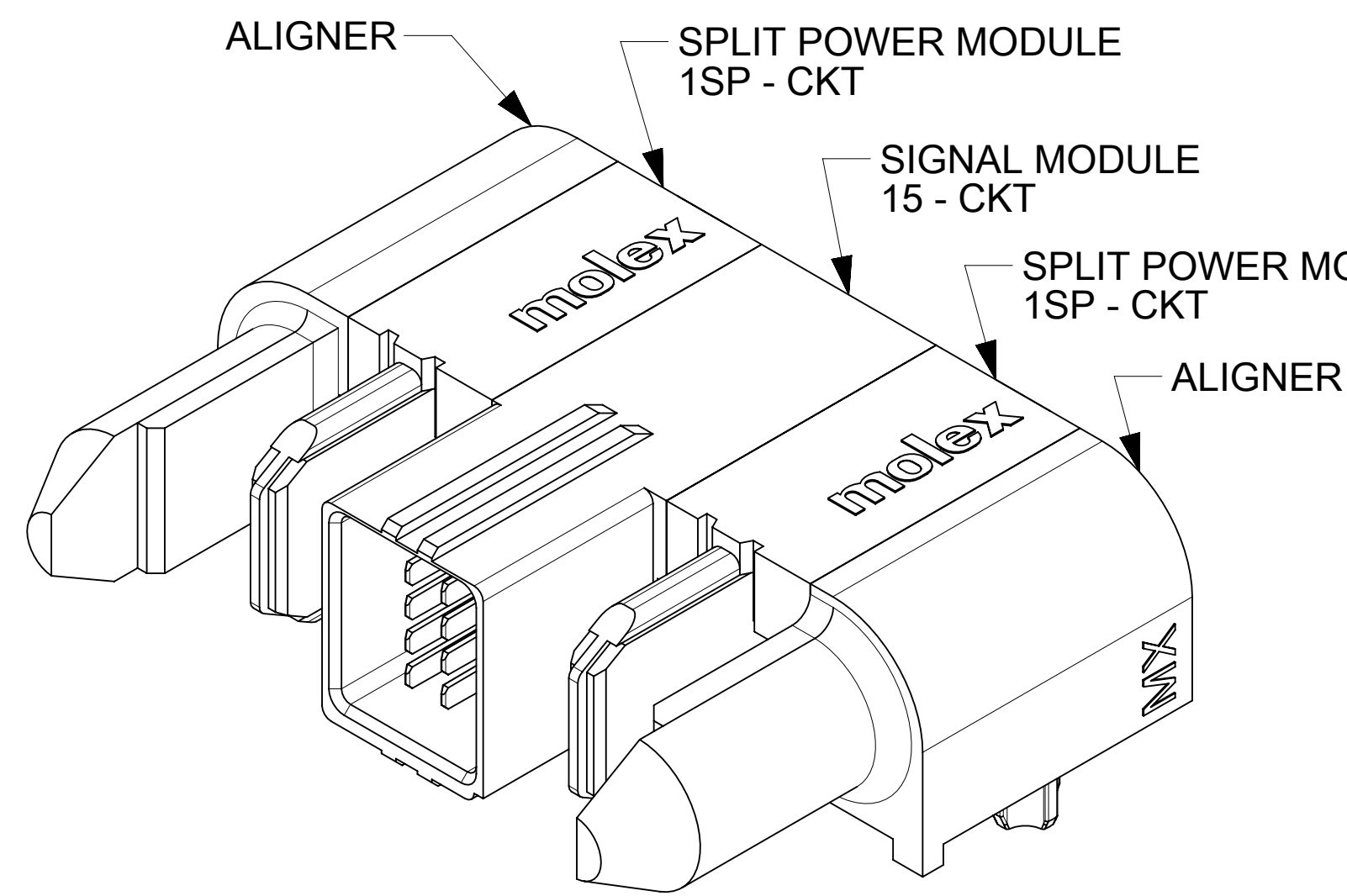
P/N: 171088-8421 (G-1SP-15S-1SP-G)
