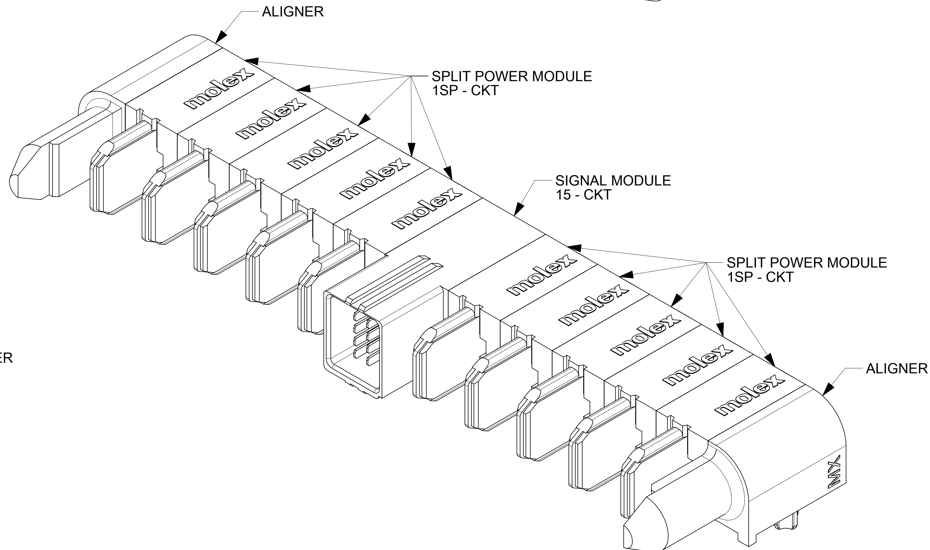
P/N: 171088-8425 (G-5SP-15S-5SP-G)
