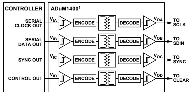
Figure 57. Isolated Interface
