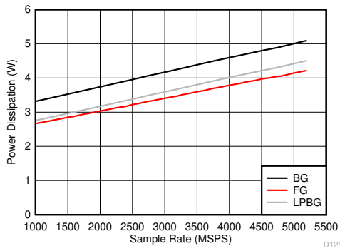
Figure 6-139. Dual Channel Mode: Power Dissipation vs Sample Rate
