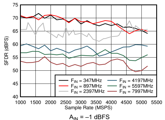
Figure 6-48. Dual Channel Mode: SFDR vs Sample Rate and Input Frequency A_{IN} = -1\text{ dBFS}
