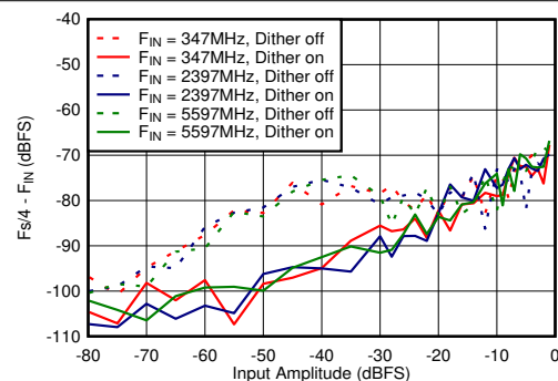
Figure 6-72. DES Mode: F_{s/4} - F_{IN} vs Input Amplitude and Dither
