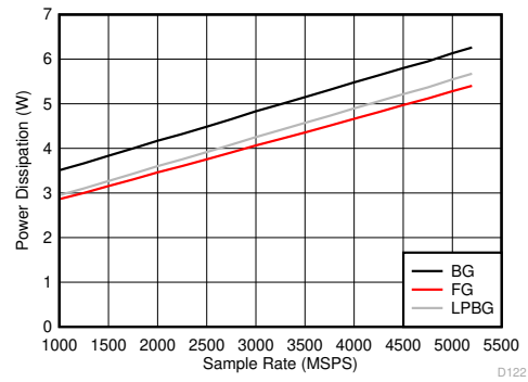
Figure 6-140. Dual Channel Mode: Power Dissipation vs Sample Rate
