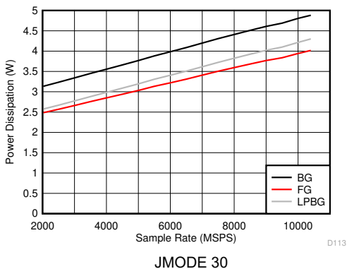
Figure 6-131. DES Mode: Power Dissipation vs Sample Rate
