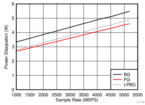
Figure 6-142. Dual Channel Mode: Power Dissipation vs Sample Rate
