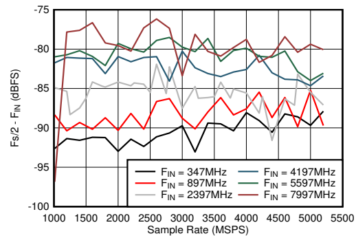
Figure 6-58. Dual Channel Mode: F_s/2 - F_{IN} vs Sample Rate and Input Frequency
