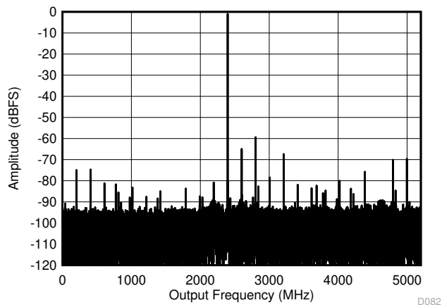
Figure 6-7. DES Mode: Single Tone FFT at 2397 MHz
