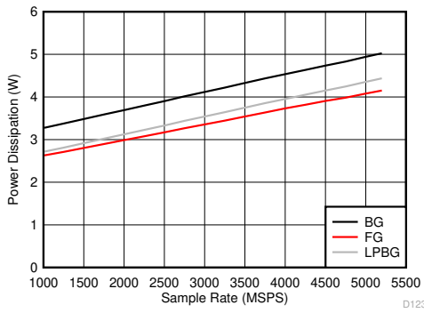
Figure 6-141. Dual Channel Mode: Power Dissipation vs Sample Rate
