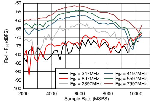
Figure 6-44. DES Mode: F_s/4 - F_{IN} vs Sample Rate and Input Frequency
