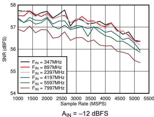
Figure 6-47. Dual Channel Mode: SNR vs Sample Rate and Input Frequency A_{IN} = -12\text{ dBFS}
