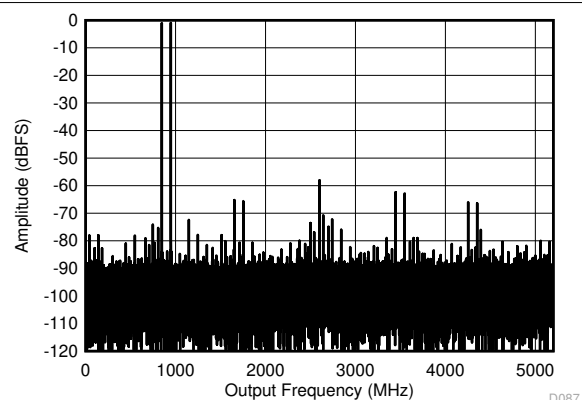
Figure 6-12. DES Mode: Two Tone FFT at 897 MHz
