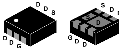
DFN2x2-6L 2EP
