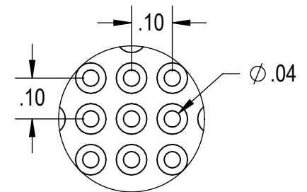
DETAIL A SCALE 3 : 1
