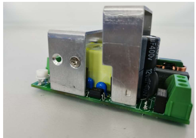
变更后，Y 电容本体颜色为深蓝 After the change, the color of some capacitors is dark blue.
