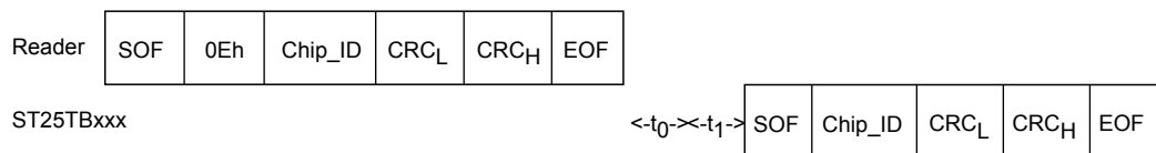
Figure 50. Select frame exchange between reader and ST25TB02K
