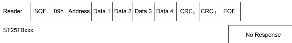
Figure 54. Write_block frame exchange between reader and ST25TB02K
