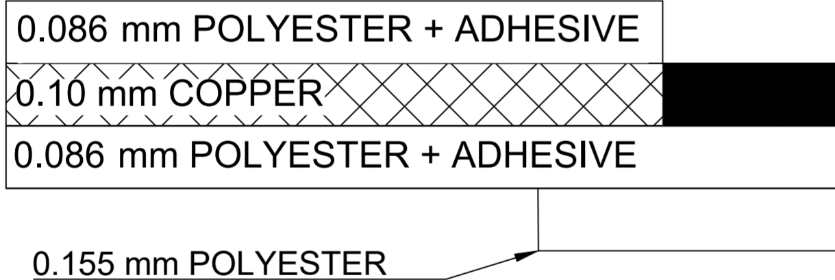
CROSS-SECTION
