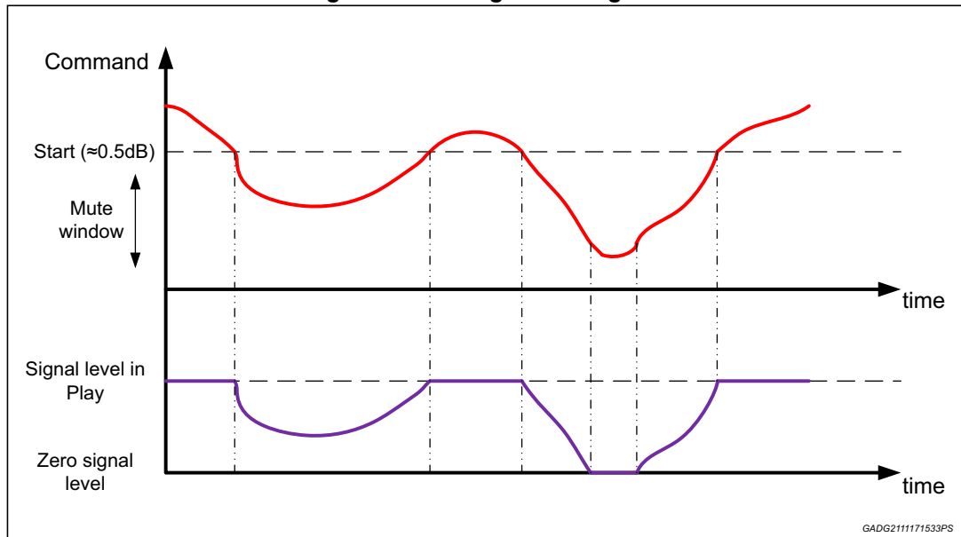
Figure 43. Analog-Mute diagram
