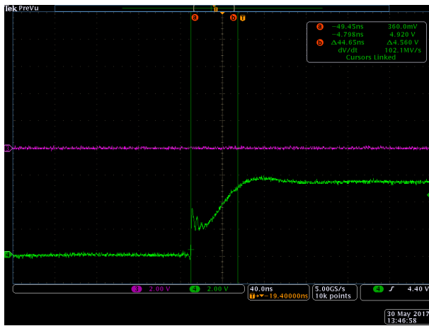
V_{DD} = V_{HB} = 6\text{ V} , HS = VSS C_{LOAD} = 10\text{ nF} Ch4 = HO
