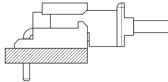
9-15極 9-15 CIRCUIT
