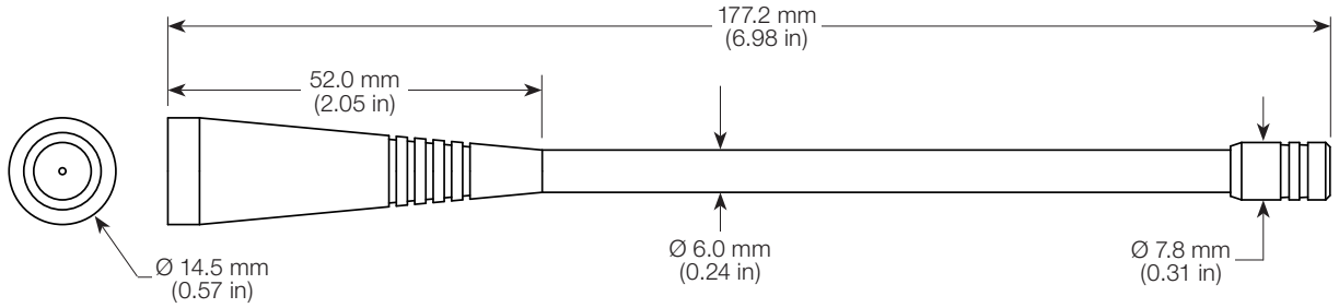
Figure6. CW 410 MHz Antenna Dimensions
