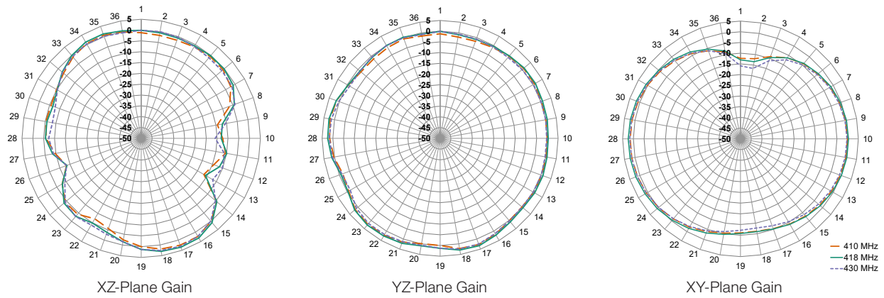
Figure8. Radiation Patterns for CW 410 MHz Antenna
