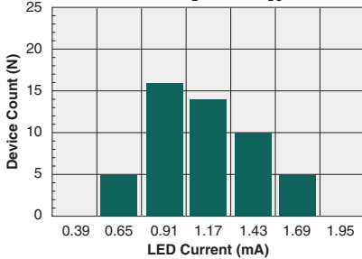
Typical I F for Switch Operation (N=50, I L =100mA DC )
