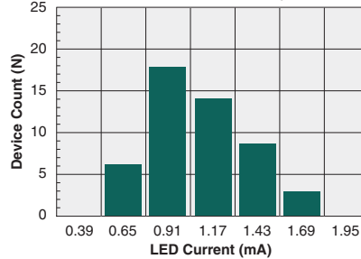
Typical I F for Switch Dropout (N=50, I L =100mA DC )
