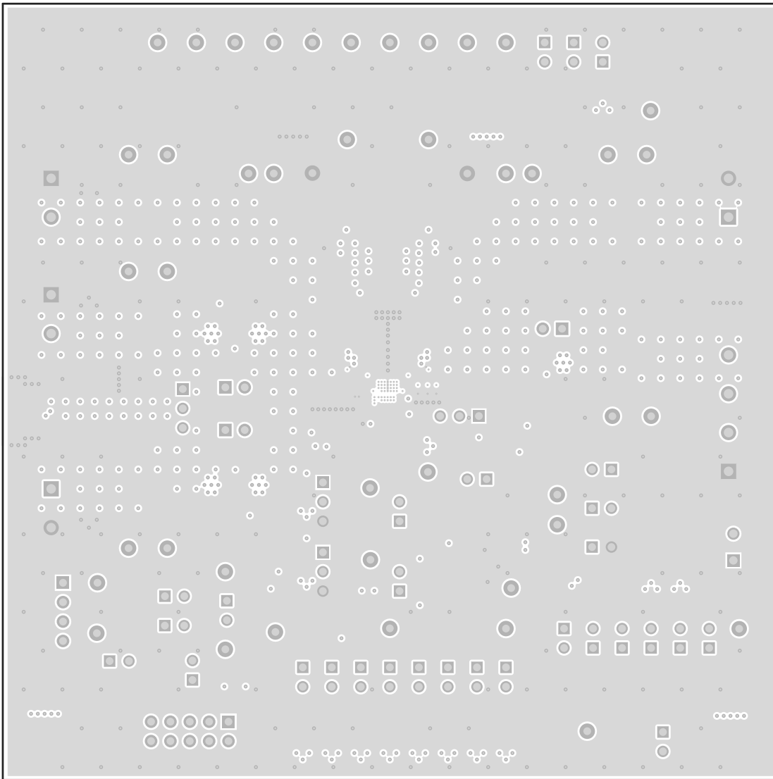
Figure 4-2. BMS027A Signal Layer 1
