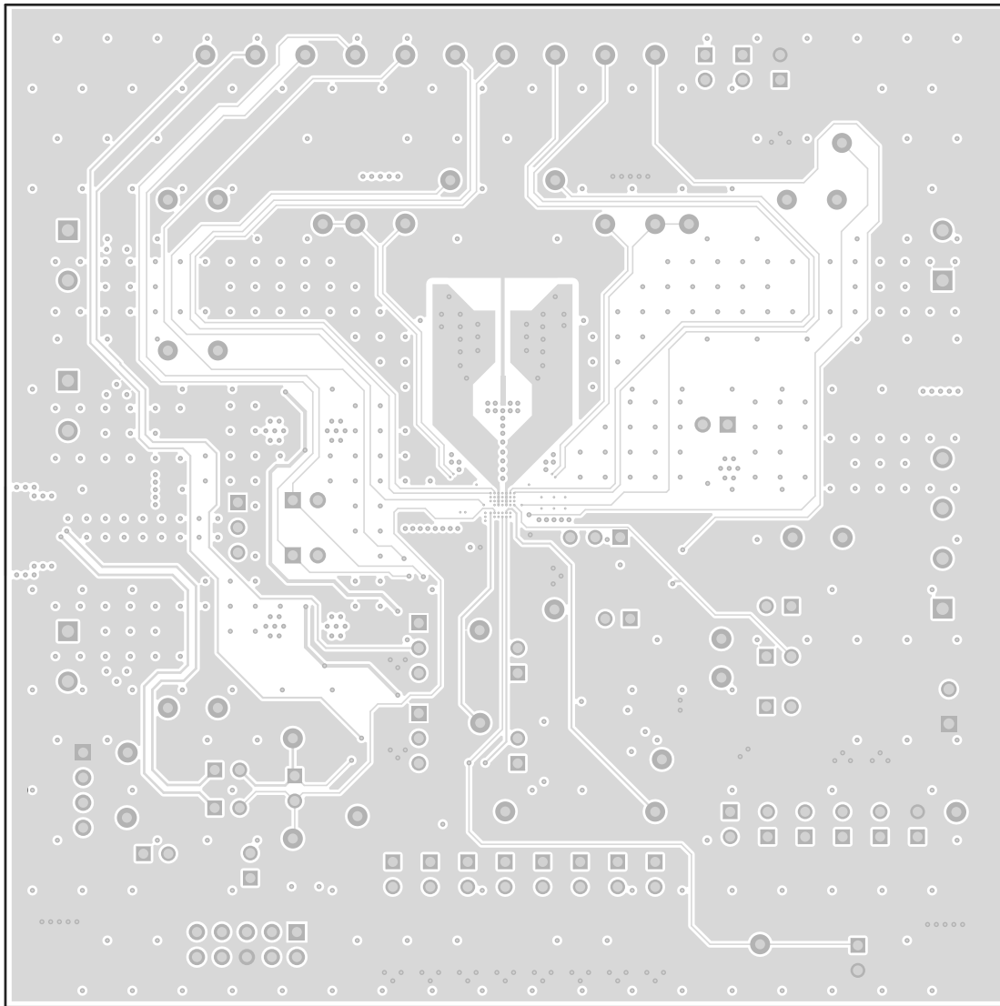
Figure 4-3. BMS027A Signal Layer 2
