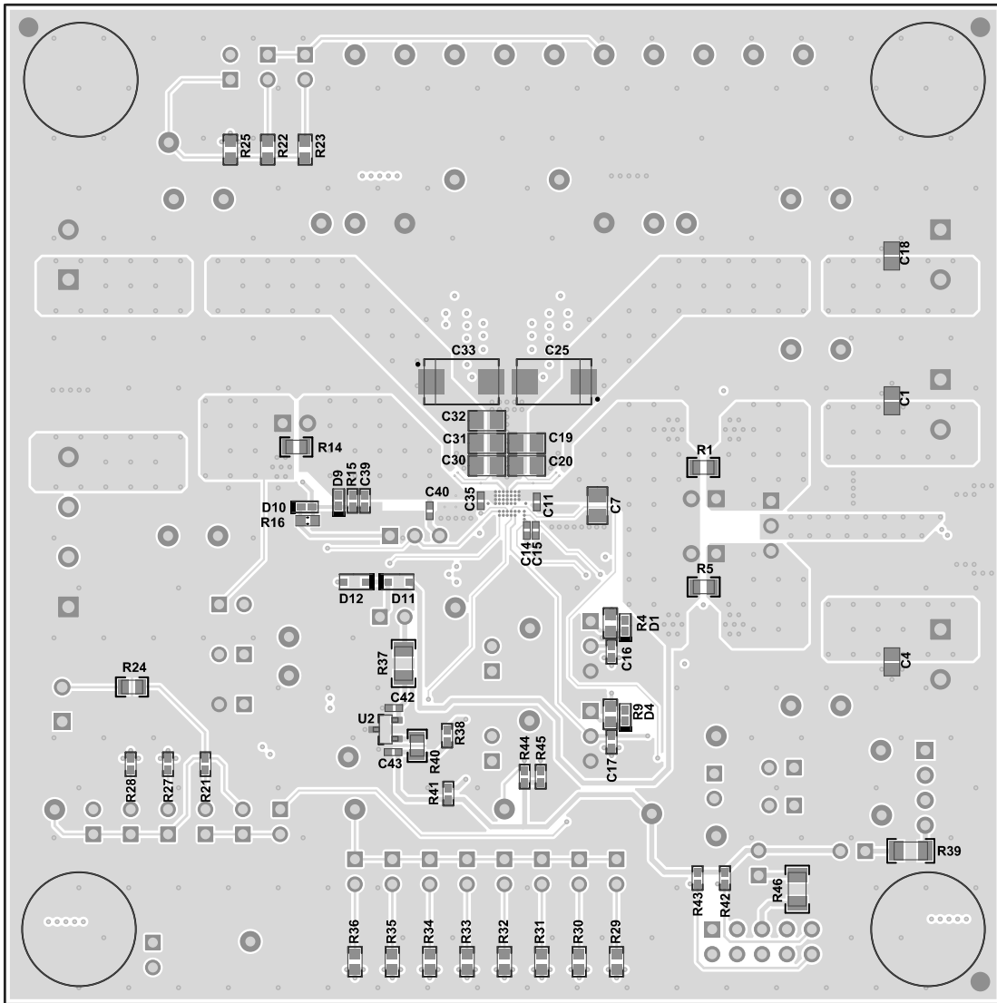
Figure 4-4. BMS027A Bottom Layer and Overlay
