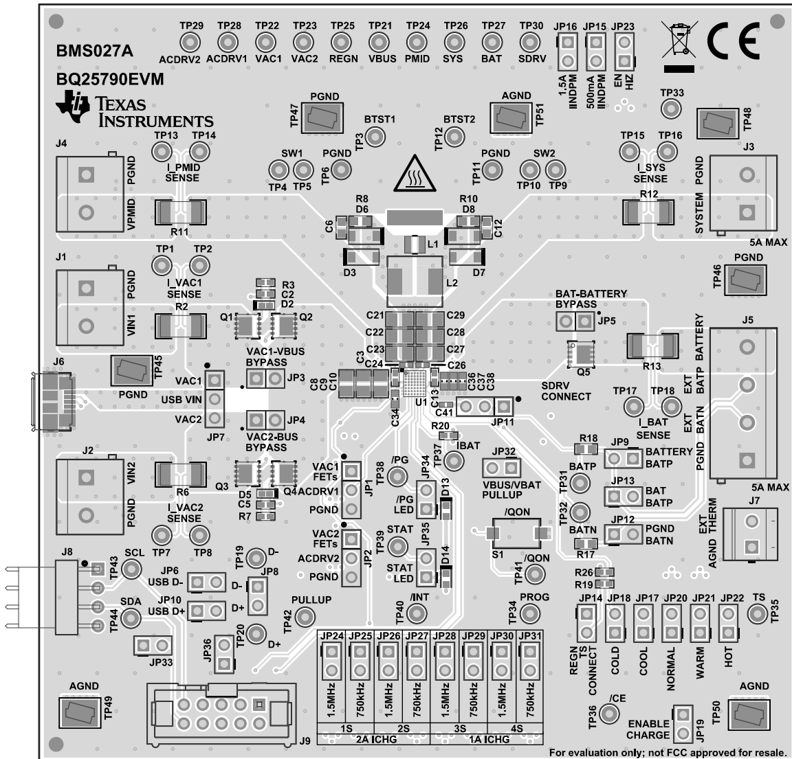
Figure 4-1. BMS027A Top Layer and Overlay
