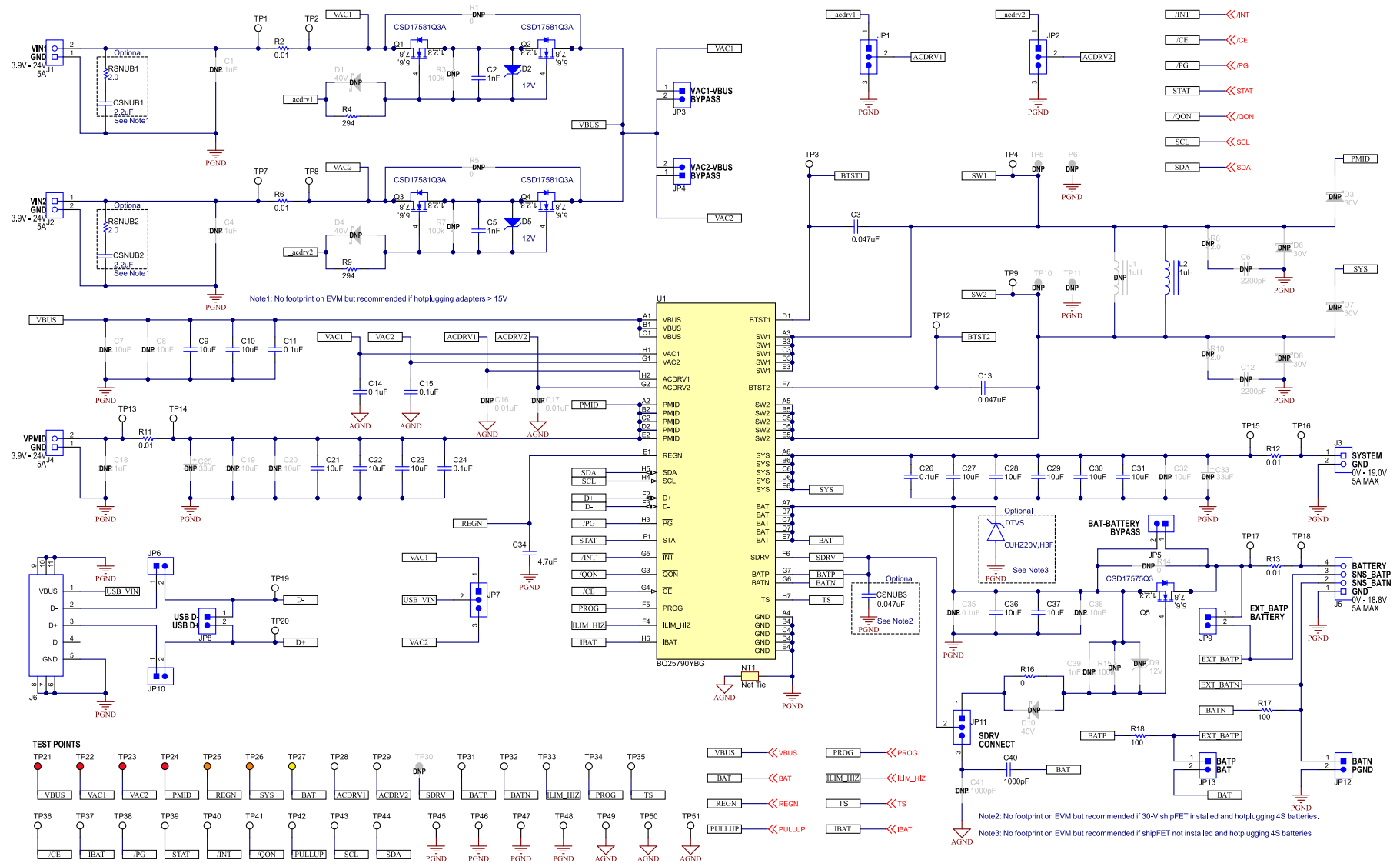
Figure 4-5. BQ25790EVM Schematic Page 1
