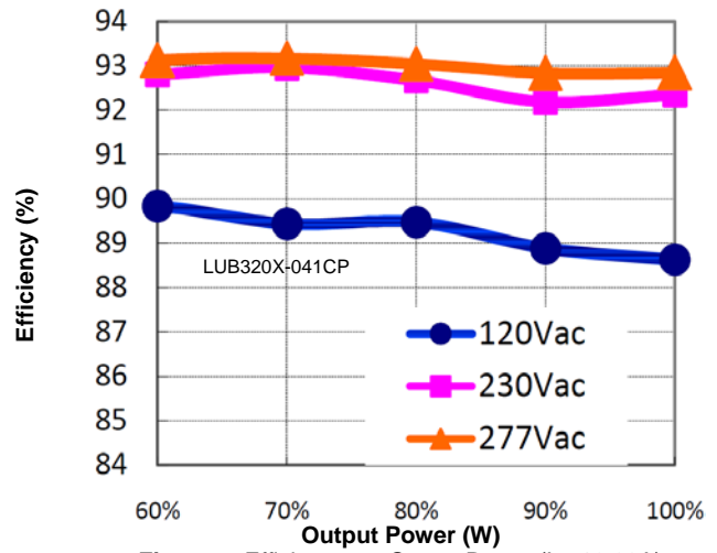
Figure 7: Efficiency vs. Output Power (Io=10.00A)
