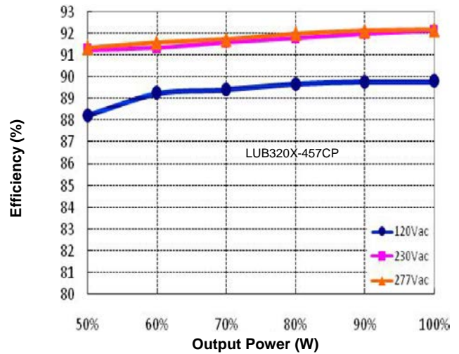
Figure 15: Efficiency vs. Output Power (Io=1.10A)
