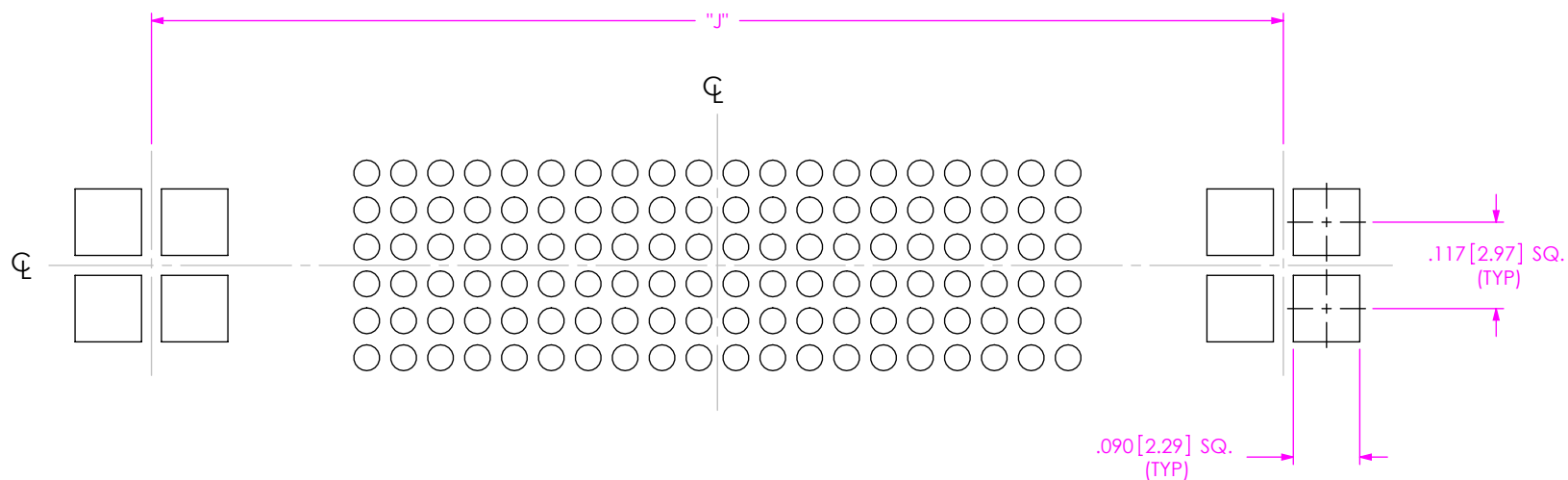
FIG 6 -LP & -PP OPTION STENCIL FOR SEAF-20-XX.X-XX-06-X-A-LP AND SEAF-20-XX.X-X-06-X (SAME AS FIG 2, EXCEPT AS SHOWN) X
