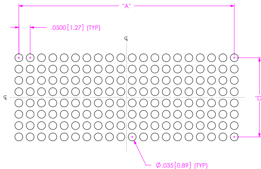
FIG 2 STENCIL FOR SEAF-20-XX.X-XX-08-X-A AND SE AFC-20-XX.X-XX-08-X-X SHOWN (ALL DIMENSIONS ARE SYMMETRIC ABOUT THE CENTERLINE.)
