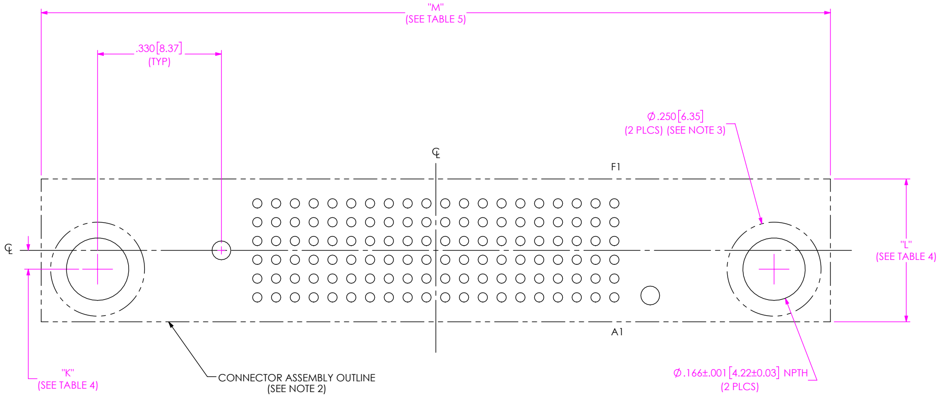
FIG 7 -GPK OPTION FOOTPRINT FOR SEAF-20-XX.X-XX-06-X-A-GPK AND SE AFC-20-XX.X-X-06-X-X-GPK SHOWN (SAME AS FIG 1, EXCEPT AS SHOWN) (NOT AVAILABLE WITH -LP & -PP OPTIONS) (STENCIL SAME AS FIG 2)
