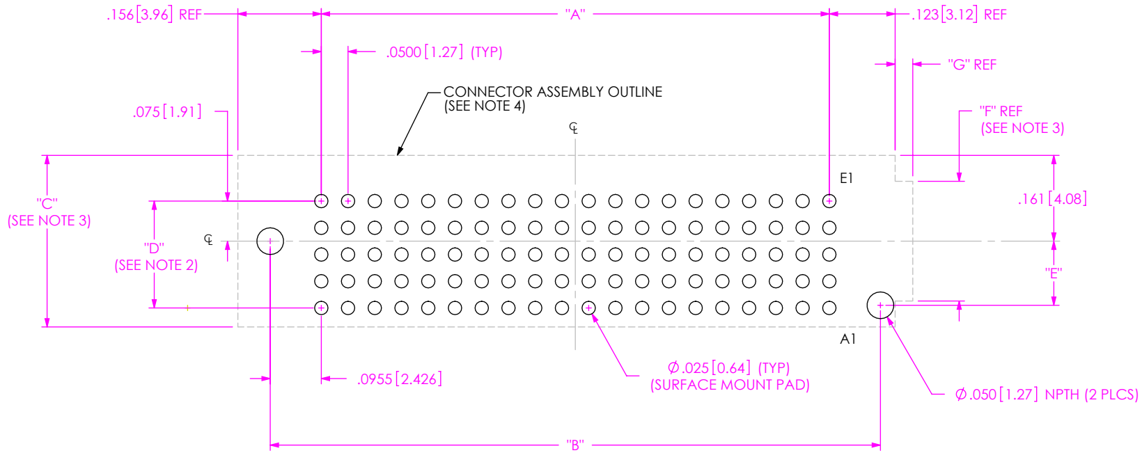
FIG 3 FOOTPRINT FOR SEAF-20-XX.X-XX-05-X-A AND SEAF-20-XX.X-X-05-X-X SHOWN
