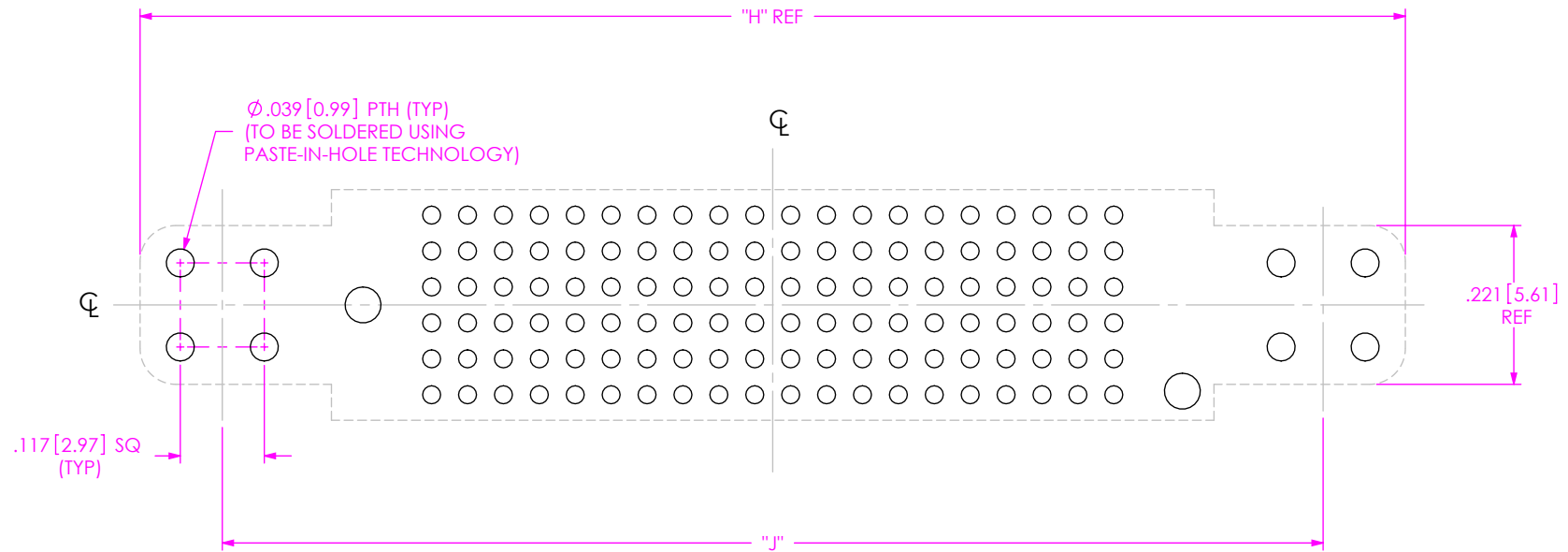
FIG 5 -LP & -PP OPTION FOOTPRINT FOR SEAF-20-XX.X-XX-06-X-A-LP AND SEAF-20-XX.X-XX-06-X SHOWN (SAME AS FIG 1, EXCEPT AS SHOWN)
