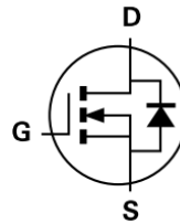
Internal Schematic
