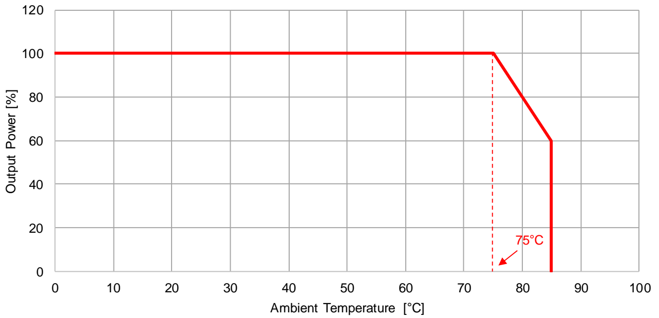
173010x35 Output Power Thermal Derating V_{IN} = 24V, I_{OUT} = 1A, f_{SW} = 520kHz
