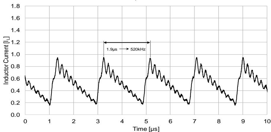
173010x35 Inductor Ripple Current V_{IN} = 24V & I_{OUT} = 500mA CCM Operation
