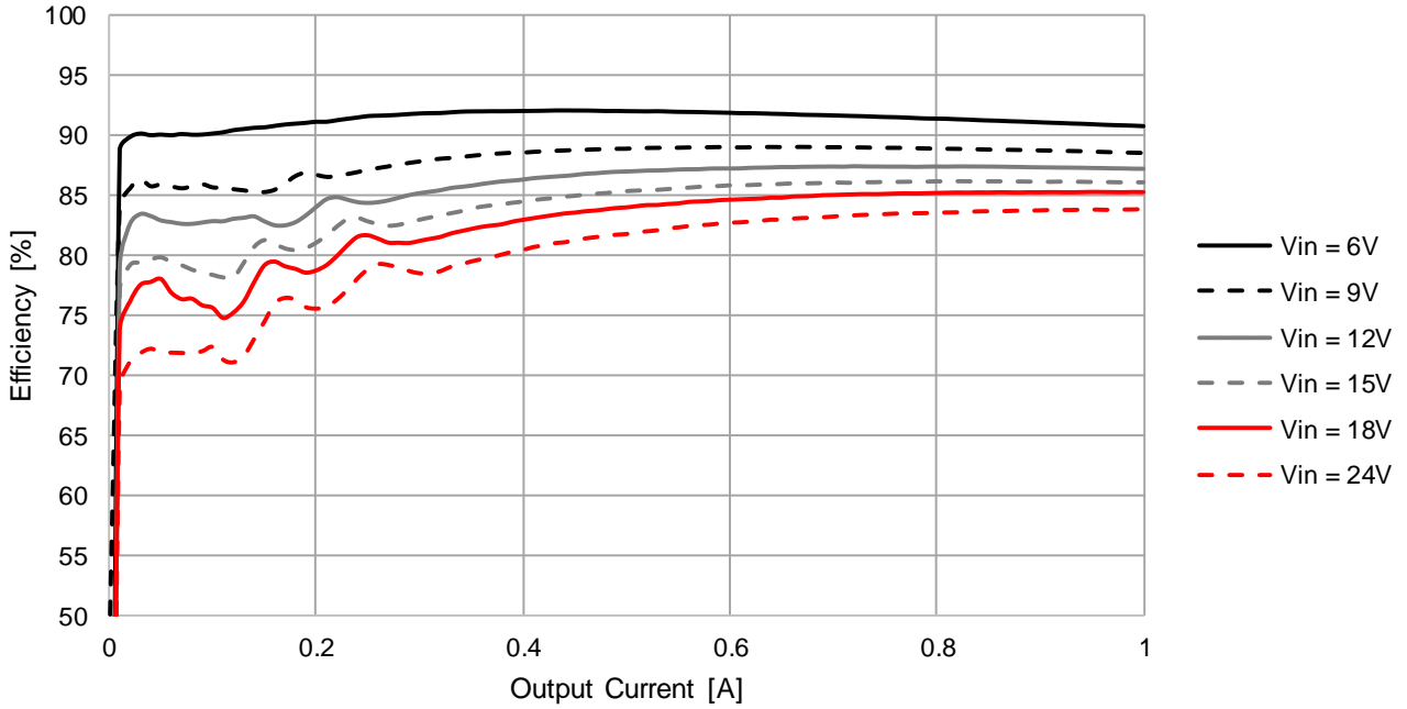
173010335 V_{OUT} = 3.3V , f_{SW} = 520kHz , T_A = 25^\circ C
