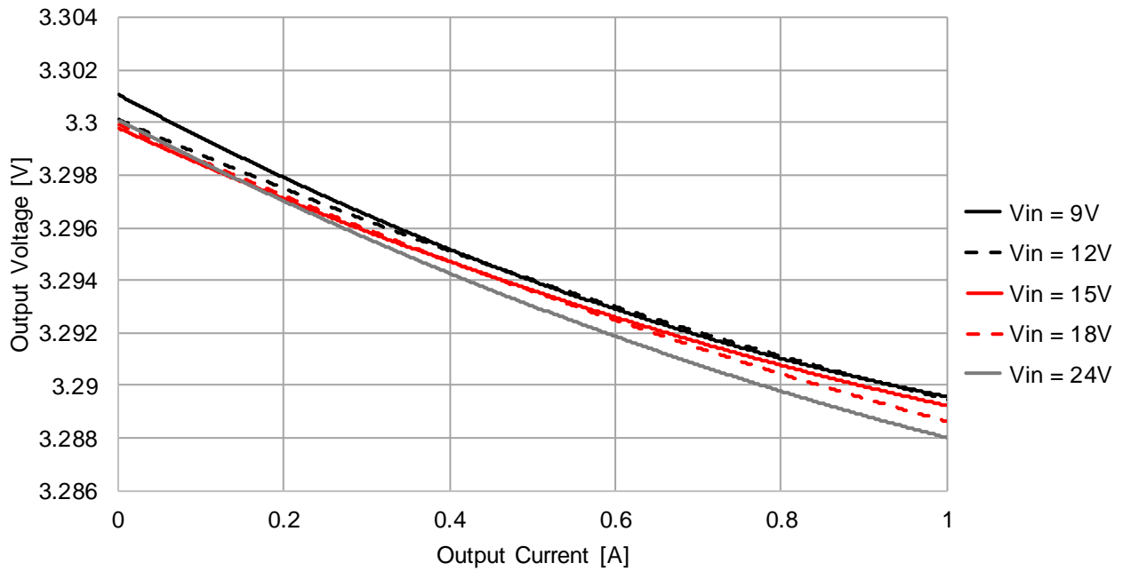
173010335 Load Regulation V_{OUT} = 3.3V , T_A = 85^\circ C
