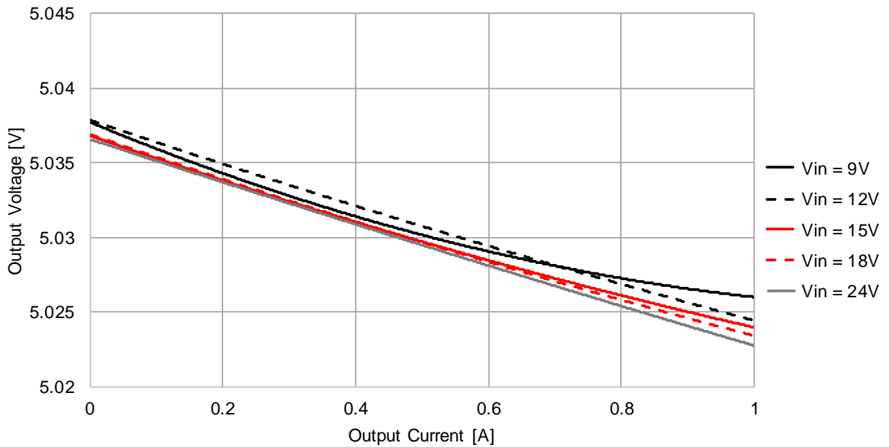
173010535 Load Regulation V_{OUT}=5V, T_A = 85^\circ C
