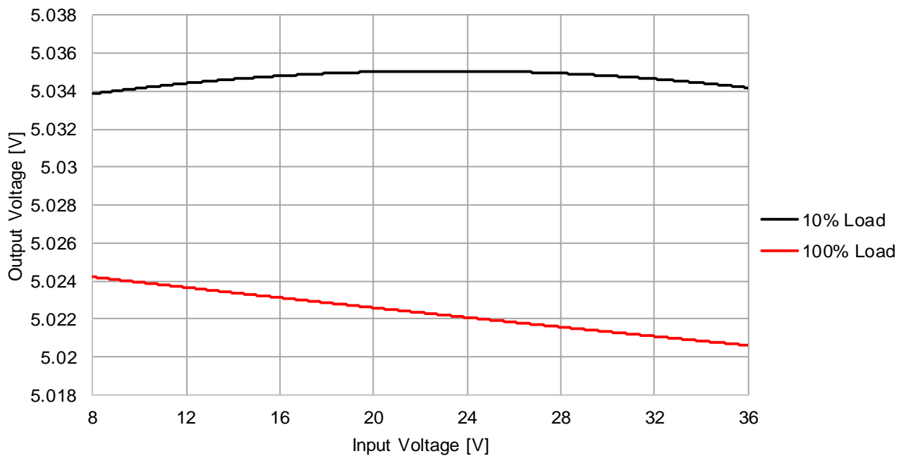
173010535 Line Regulation V_{OUT} = 5V , T_A = 85^\circ C
