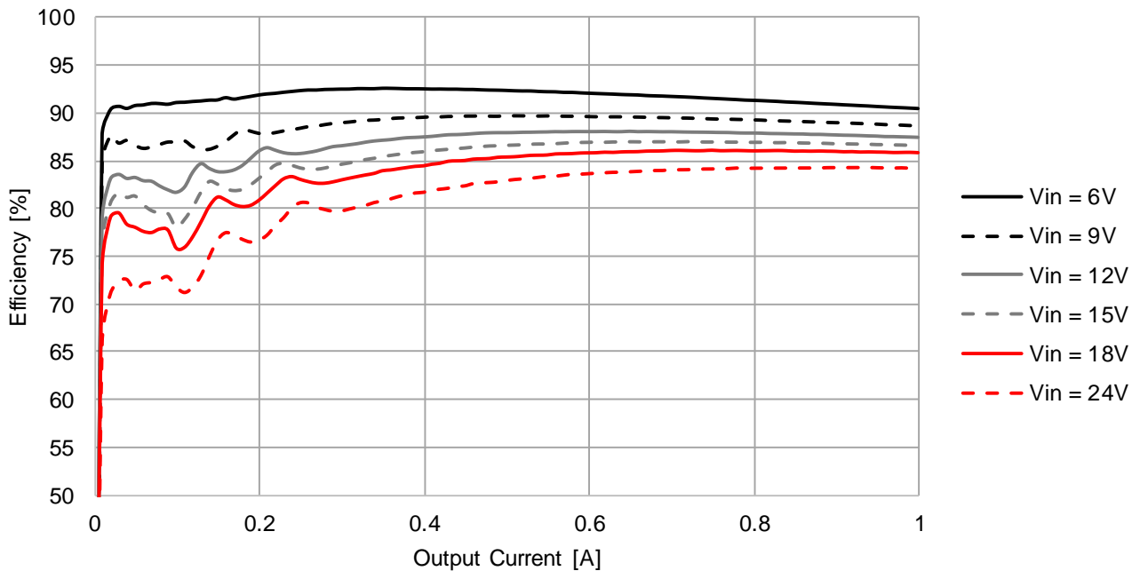
173010335 V_{OUT} = 3.3V , f_{SW} = 520kHz , T_A = 85^\circ C
