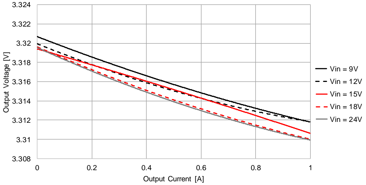
173010335 Load Regulation V_{OUT} = 3.3V , T_A = 25^\circ C
