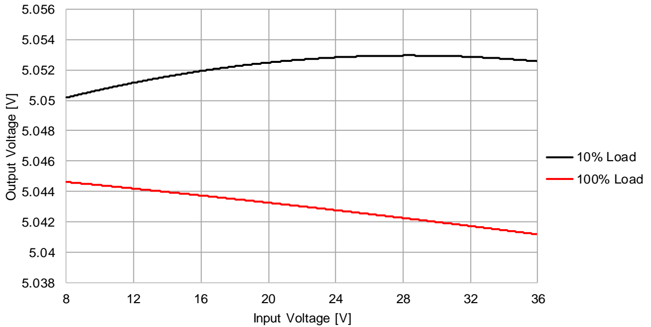
173010535 Line Regulation V_{OUT} = 5V , T_A = 25^\circ C
