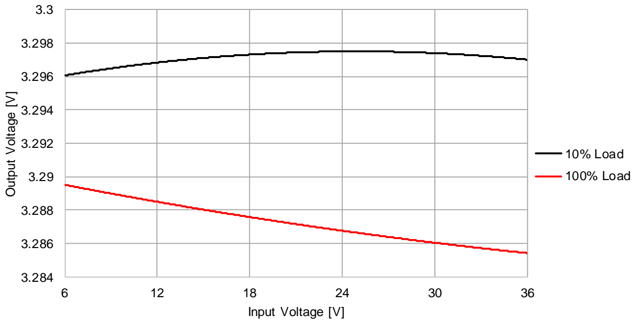
173010335 Line Regulation V_{OUT} = 3.3V , T_A = 85^\circ C
