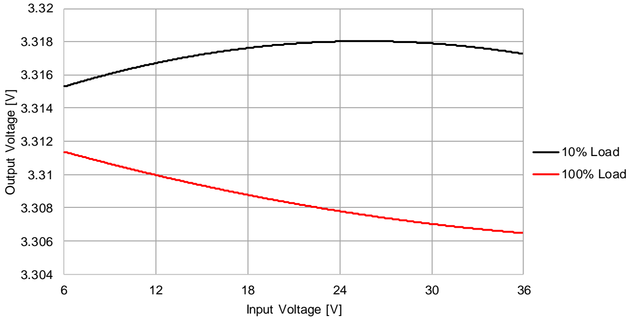
173010335 Line Regulation V_{OUT} = 3.3V , T_A = 25^\circ C
