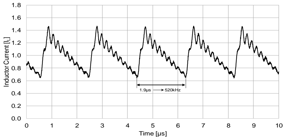
173010x35 Inductor Ripple Current V_{IN} = 24V & I_{OUT} = 1A CCM Operation
