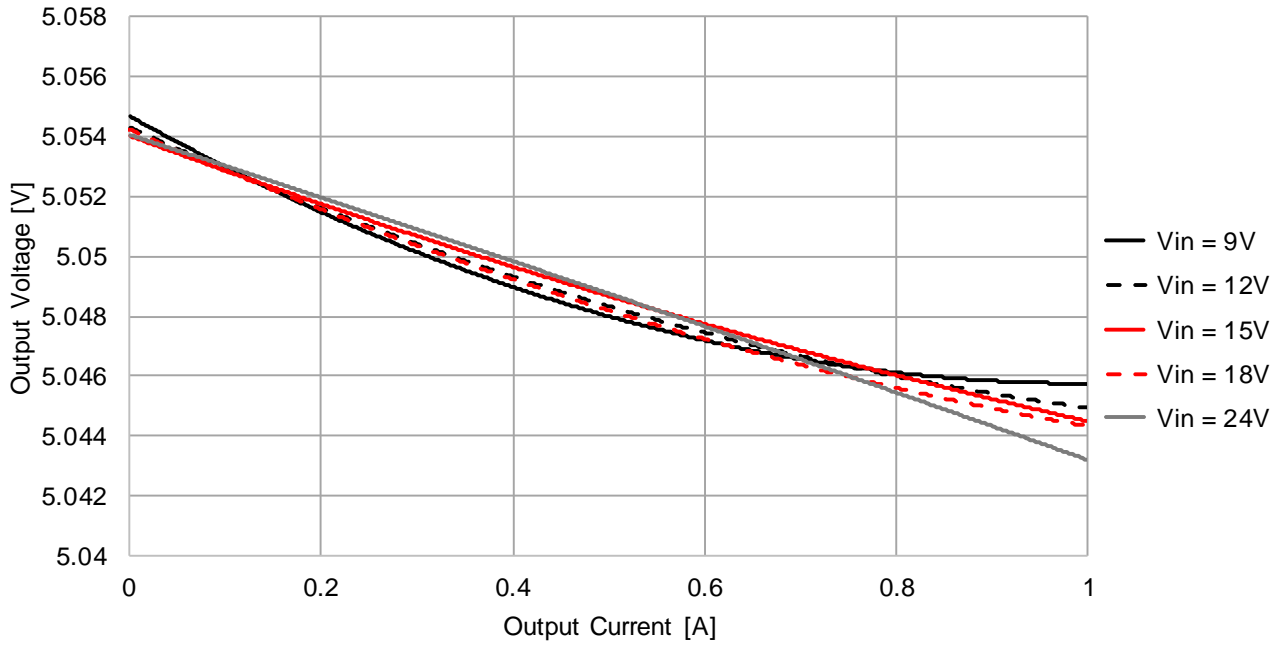
173010535 Load Regulation V_{OUT}=5V, T_A = 25^\circ C
