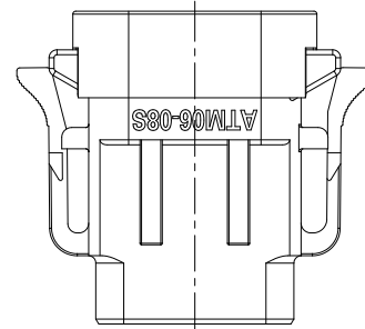
P/N ATM06-08SC-SF1GN KEY-C CONFIGURATION STANDARD COLOR: GREEN
