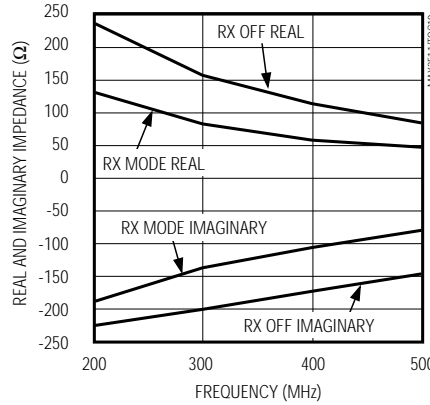
RXIN DIFFERENTIAL INPUT IMPEDANCE vs. FREQUENCY
