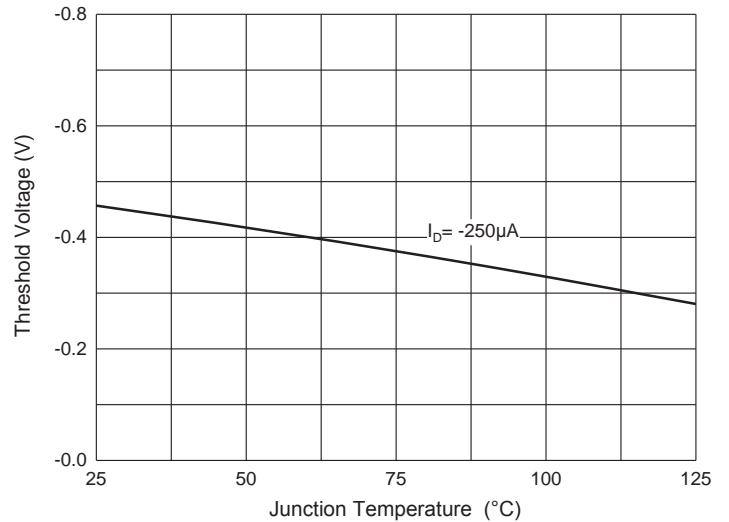
Fig. 12 - Threshold Voltage
