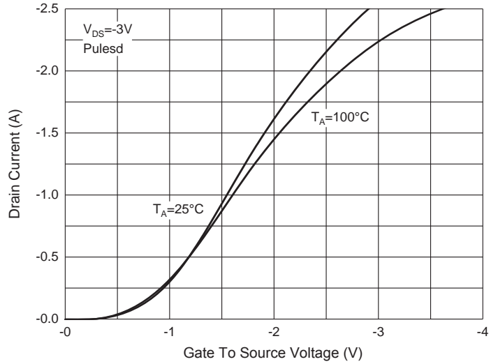
Fig. 8 - Transfer Characteristics
