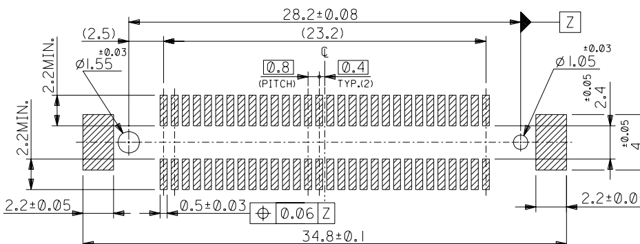
推奨基板寸法 RECOMMENDED PCB PATTERN LAYOUT
