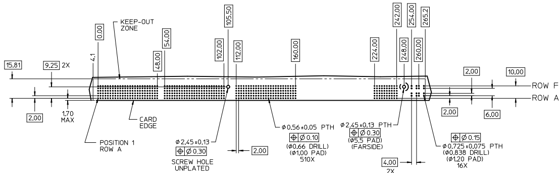
DAUGHTERCARD HOLE PATTERN (CONNECTOR SIDE)
