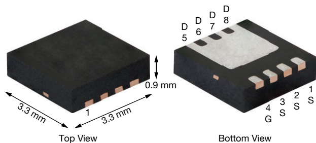
PowerPAK® 1212-8SH
