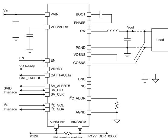
Simplified Schematic
