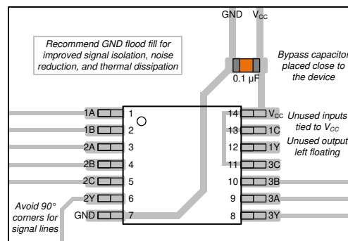
Figure 11. Example layout for the SN74HCS11
