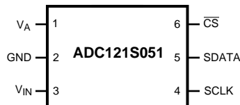
Figure 1. 6-Lead SOT-23 or WSON See DBV or NGF Package
