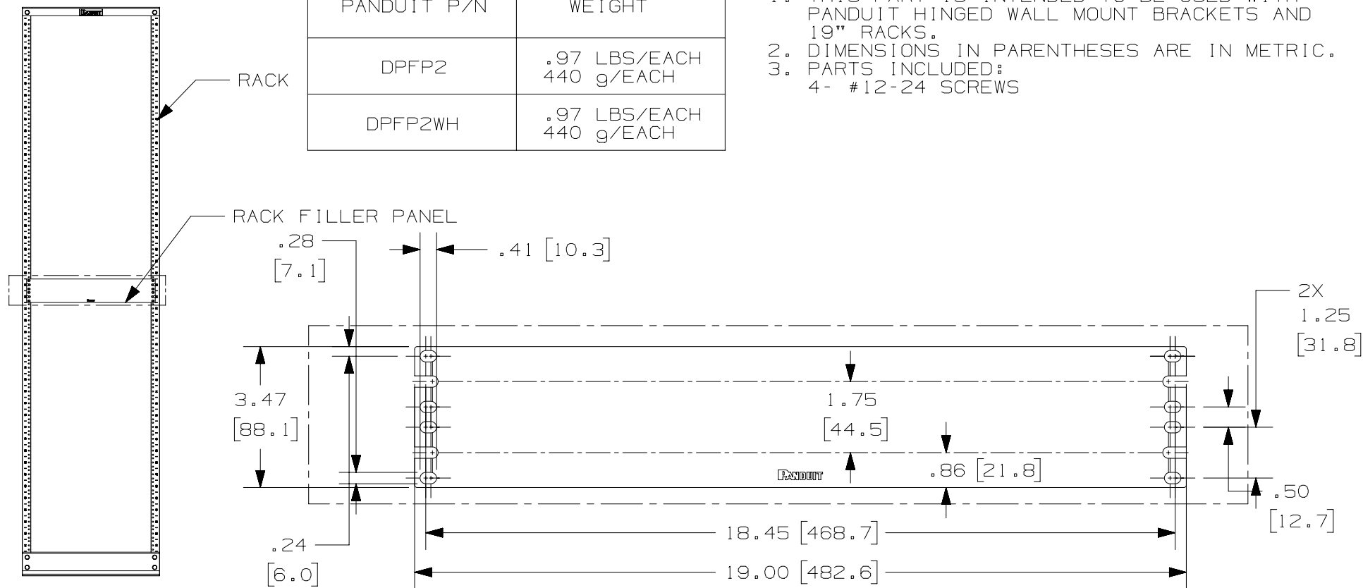
DETAIL VIEW
