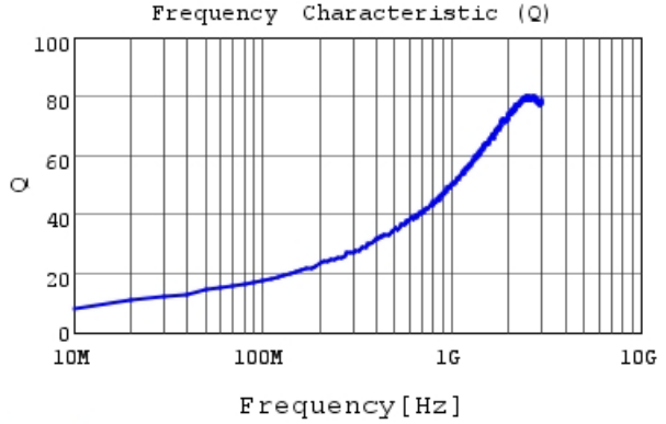
LQG15WZ2N5S02 Q
