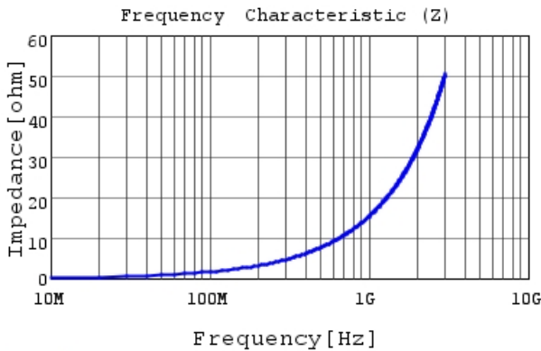
LQG15WZ2N5S02 |Z|
