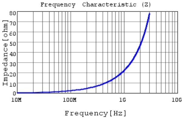
LQG15WZ3N5S02 |Z|
