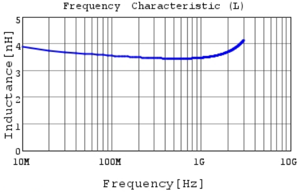
LQG15WZ3N5S02 L
