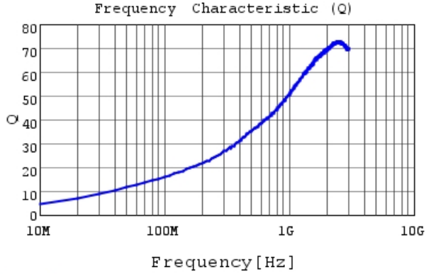
LQG15WZ3N5S02 Q
