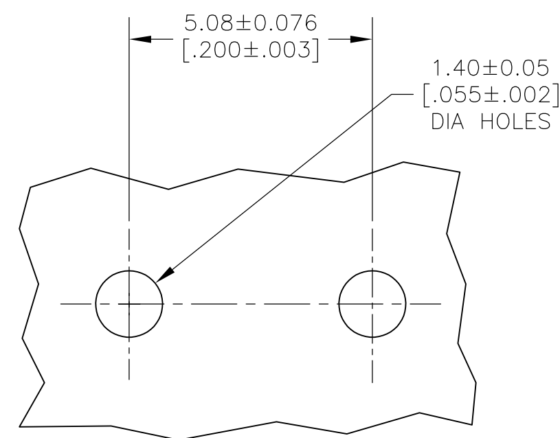
P.C. BOARD HOLES
