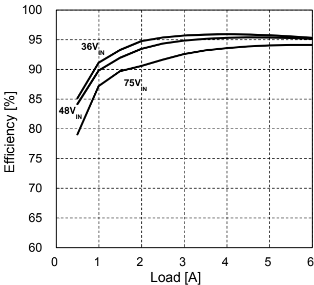
Fig.2: Efficiency vs. load current and input voltage for power module mounted horizontally with airflow 400LFM (2.0m/s) and T a =25°C.
