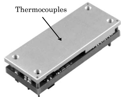
Fig. G: Location of thermocouples for thermal testing (With base-plate)
