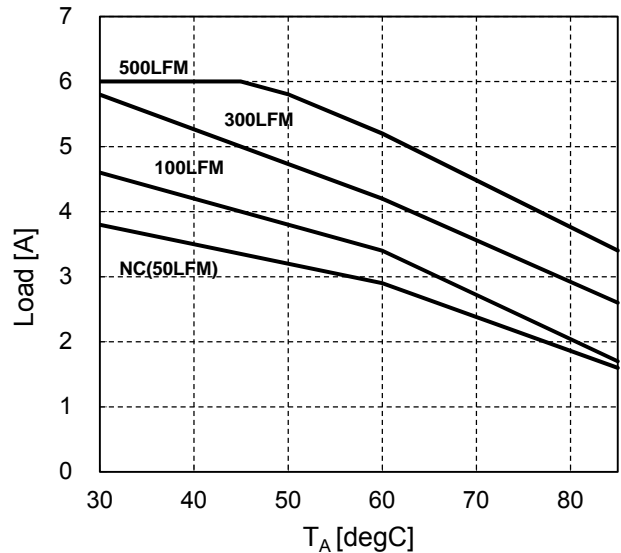
Fig.1-b: Available load current vs. ambient temperature and airflow rates for V IN =48V without base-plate (open frame). Airflow is from Pin 3 to Pin 1. Maximum component temperature ≤ 125°C
