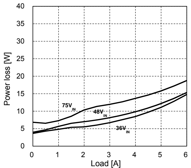
Fig.3: Power Loss vs. load current and input voltage for power module mounted horizontally with airflow 400LFM (2.0m/s) and T a =25°C.
