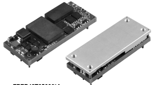
FPER48T05006*A (Open frame version)
