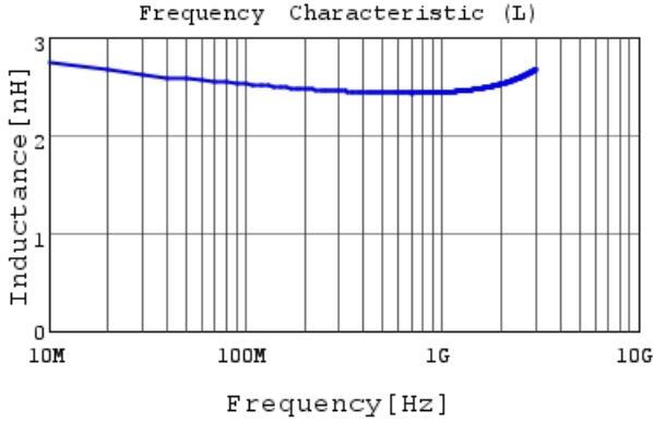
LQG15WH2N5S02 L
