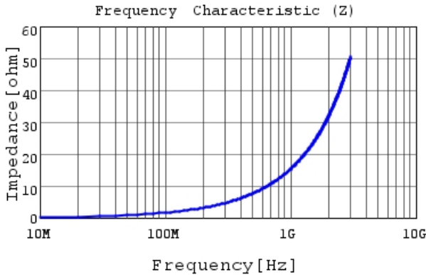
LQG15WH2N5S02 |Z|
