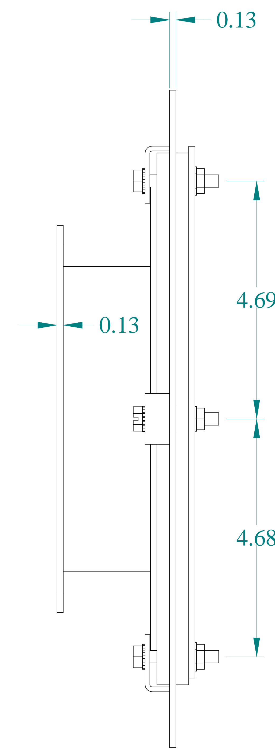
SIDE VIEW
