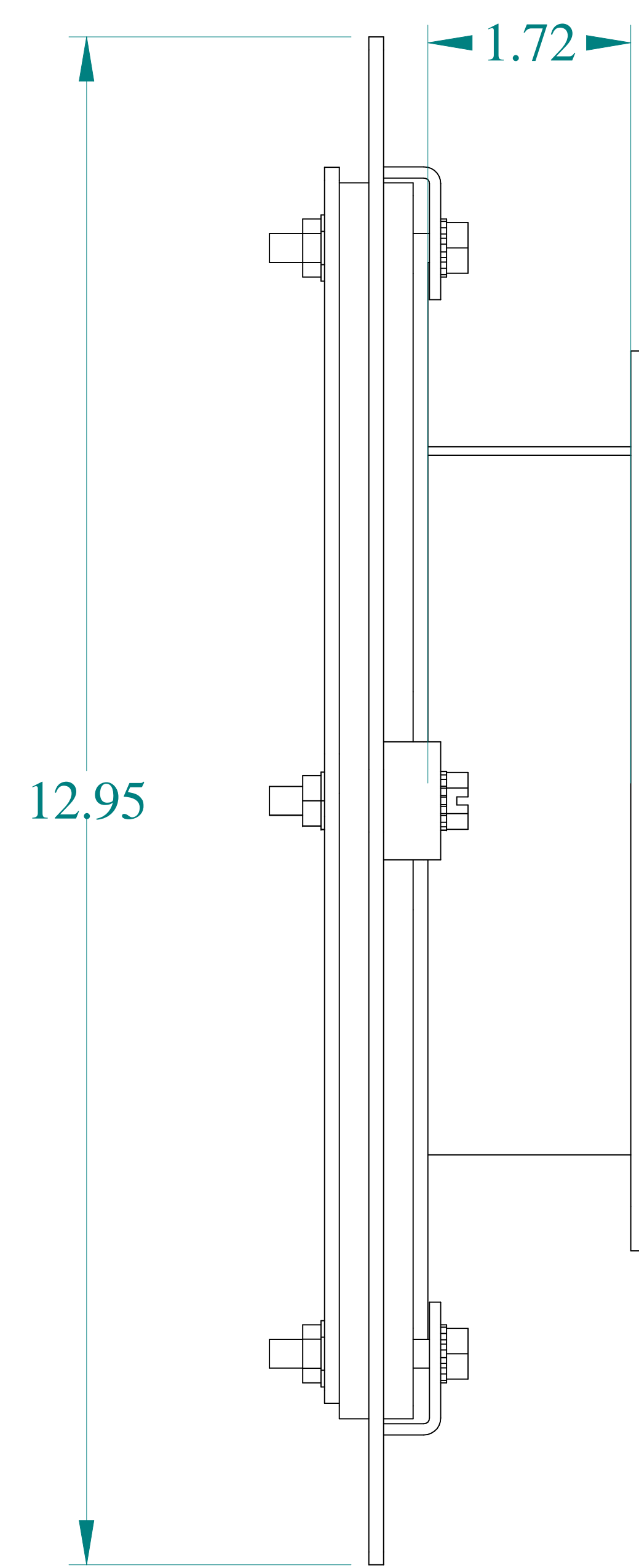
SIDE VIEW
