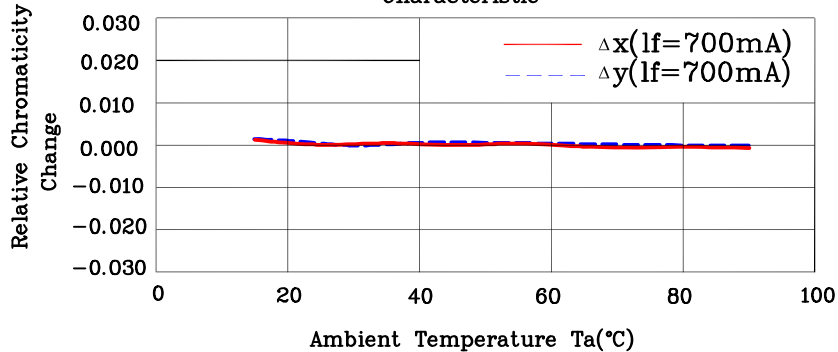
Ambient Temperature Ta-Relative Chromaticity Change Characteristic
