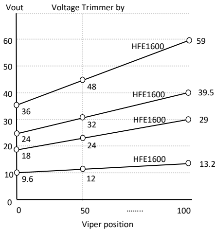
Figure 3–9: Output Voltage Limits
