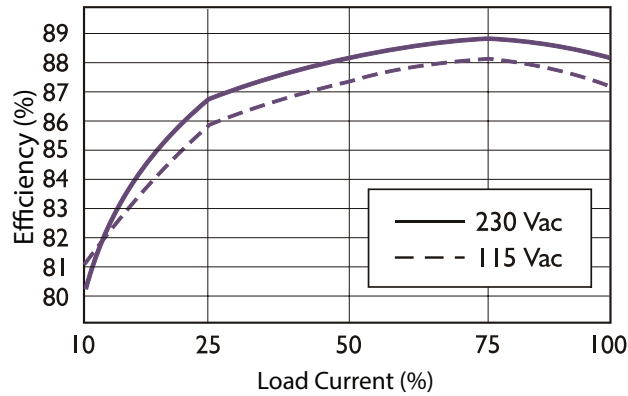
PPDRB-300-24 Efficiency Curve (Efficiency vs. Load Current)
